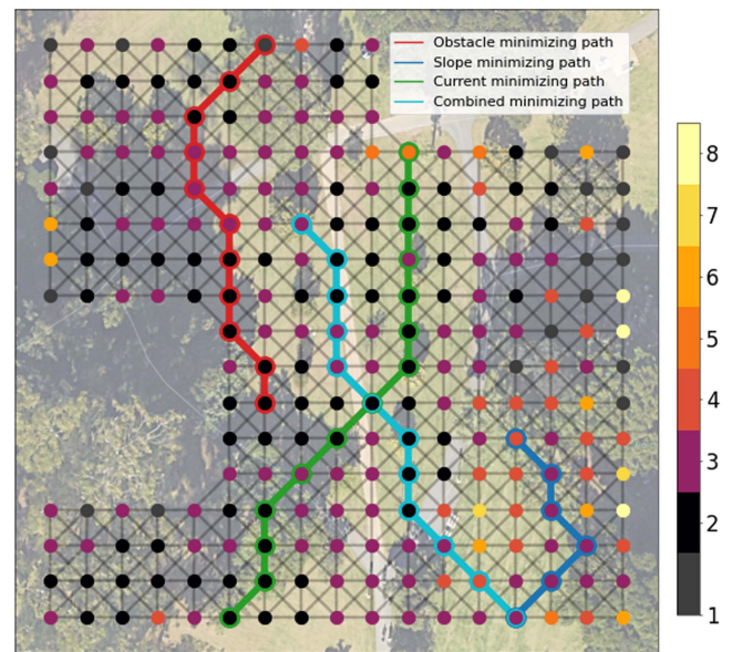
Fig. 4. Costmap for all costs added and normalized after learning. Nodes are colored according to the mean of the delays D from other nodes. Example paths minimizing current drawn, obstacles encountered, and steepness are colored green, red, and blue, respectively.
