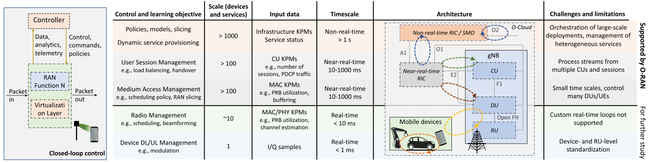
Fig. 5. Closed-loop control in the Open RAN architecture. Based on [9] and [19].
