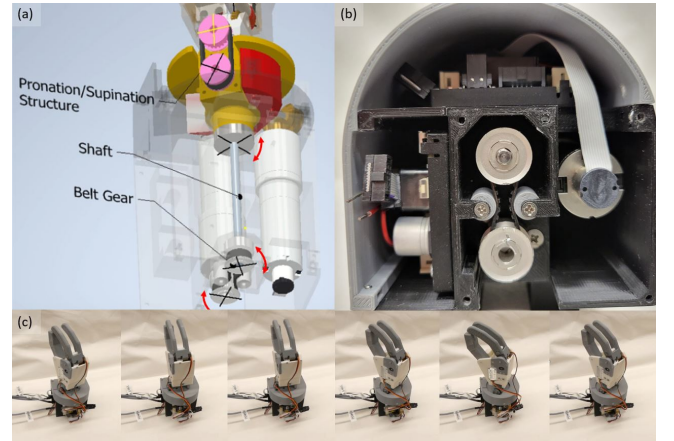
Fig. 6. (a) The CAD model shows the PS mechanism motions indicative by the red arrows (b) The PS motion belt and gears with idle rollers to tension the belt (c) PS Motion of the UBArm with max range of 15° pronation and 55° Supination
