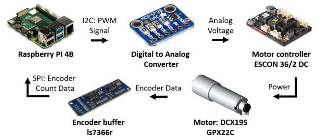
Fig. 2. Hardware diagram of the UBArm: Raspberry Pi sends PWM signal to DAC to control the ESCON motor controllers using Analog voltage. The motor position is tracked from the encoder feedback using the encoder buffer.
