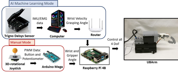
Fig. 3. Two System configuration modes: AI Machine Learning Mode predicting wrist velocity and gripper angle. The Manual Mode uses a 3-potentiometer joystick to map out wrist and gripper angle
