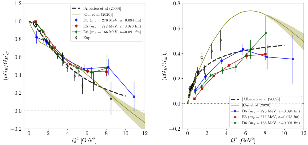
Fig. 7 Ratio of proton (left) and neutron (right) Sachs form factors \mu G_E/G_M , compared to phenomenological fits of experimental data [16] and quark+diquark Faddeev equation calculations [2]. Disconnected quark contractions are neglected
