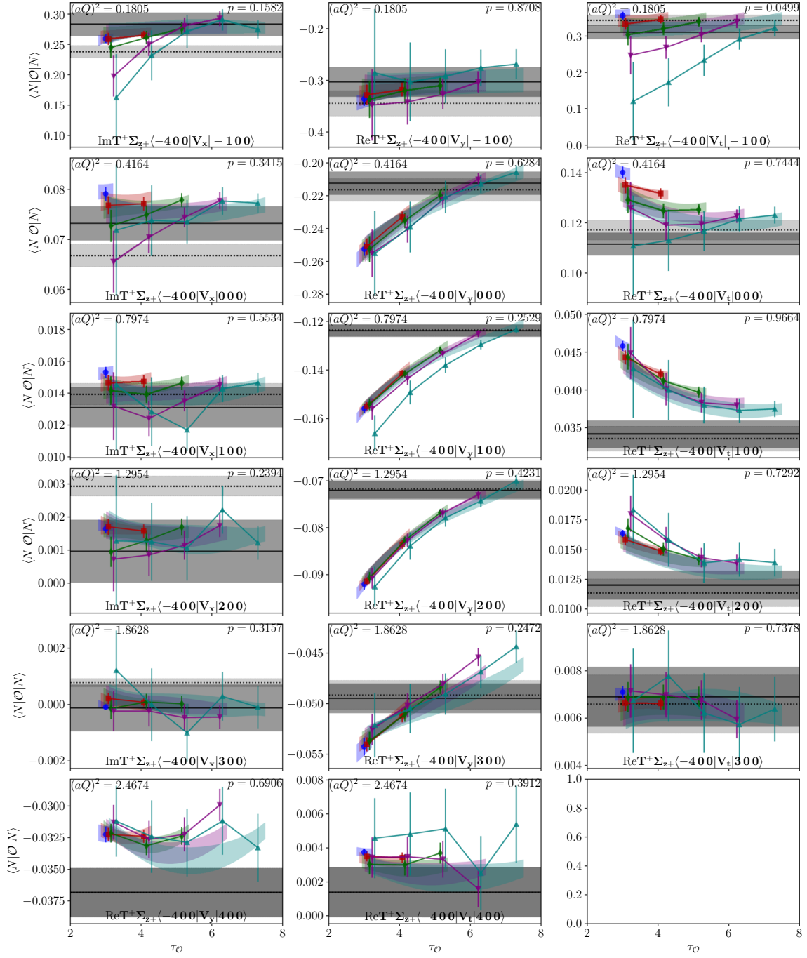
Fig. 4 Fits to the nucleon three-point functions (3) for the D5 ensemble. The colored bands show fits to Eq. (3), the dark-gray bands are the ground-state values A_{00} from these fits, and the light-gray bands are overdetermined fits of these matrix elements to the form factors F_{1,2}(Q^2)
