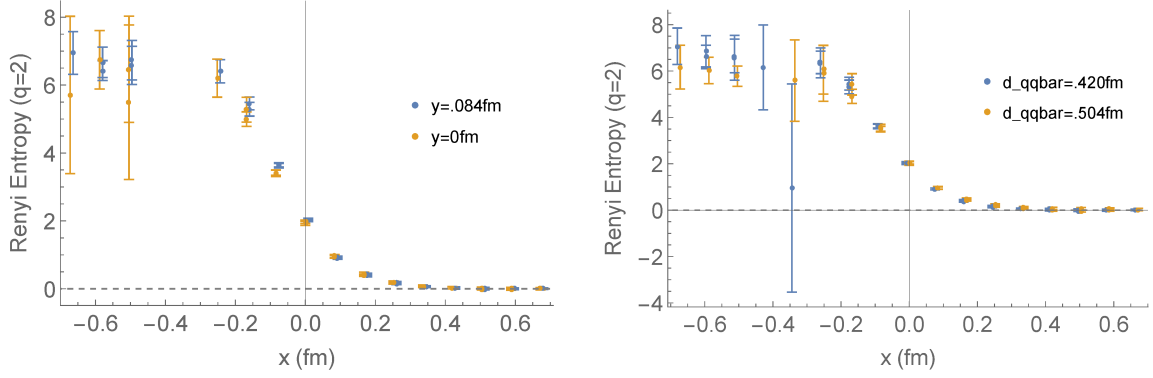
Figure 5: The excess entanglement entropy of the flux tube (partially) cross-cut by region \mathcal{A} with w = a = 0.084 fm, see Fig. 2 for explanation. (Left) dependence on the position y relative to the center of region \mathcal{A} . The Q\bar{Q} distance is d_{Q\bar{Q}} = 5a = 0.420 fm. (Right) dependence on the distance between Q and \bar{Q} . The data points are offset horizontally for clarity.
