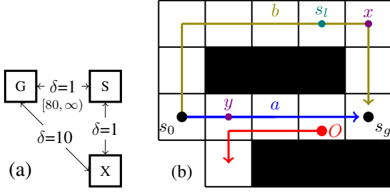
Figure 2: RTSIPP examples that defeat scalar learning.
