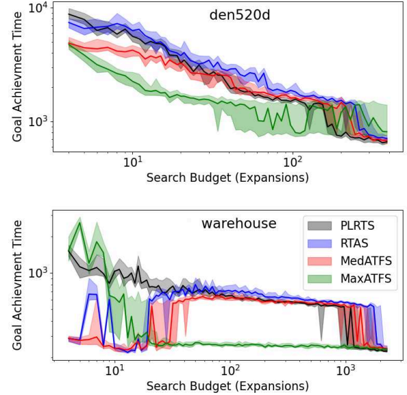
Figure 4: Goal achievement time results, median (solid line), 95% confidence interval(filled), limited to 10000 time units.
