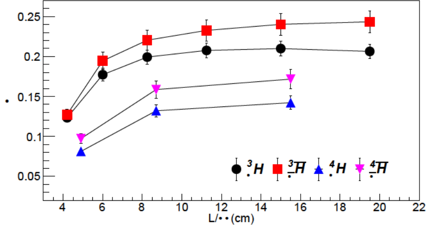
Figure 2: Reconstruction efficiency as a function of L/(\beta\gamma) obtained from the embedding Monte Carlo technique. Hypernuclei have stricter topological cuts than antihypernuclei to suppress knock-out {}^3\text{He} and {}^4\text{He} , resulting in lower efficiencies.
