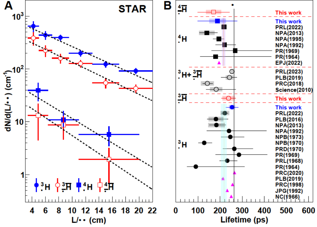
Figure 4: (A) {}^3_\Lambda\text{H} , {}^3_{\bar\Lambda}\text{H} , {}^4_\Lambda\text{H} and {}^4_{\bar\Lambda}\text{H} yields versus L/\beta\gamma . The vertical error bars represent the statistical uncertainties only. (B) Our measured {}^3_\Lambda\text{H} , {}^3_{\bar\Lambda}\text{H} , {}^4_\Lambda\text{H} and {}^4_{\bar\Lambda}\text{H} lifetimes compared with world data 7,11,28,31–42 and theoretical predictions 43–48 (solid triangles). Error bars and boxes show statistical and systematic uncertainties, respectively. Solid vertical lines with shaded regions represent the average lifetimes of {}^3_\Lambda\text{H} and {}^4_\Lambda\text{H} and their corresponding uncertainties. These are calculated from previous results by a maximum-likelihood fit. The vertical gray line shows the lifetime of the free \Lambda .
