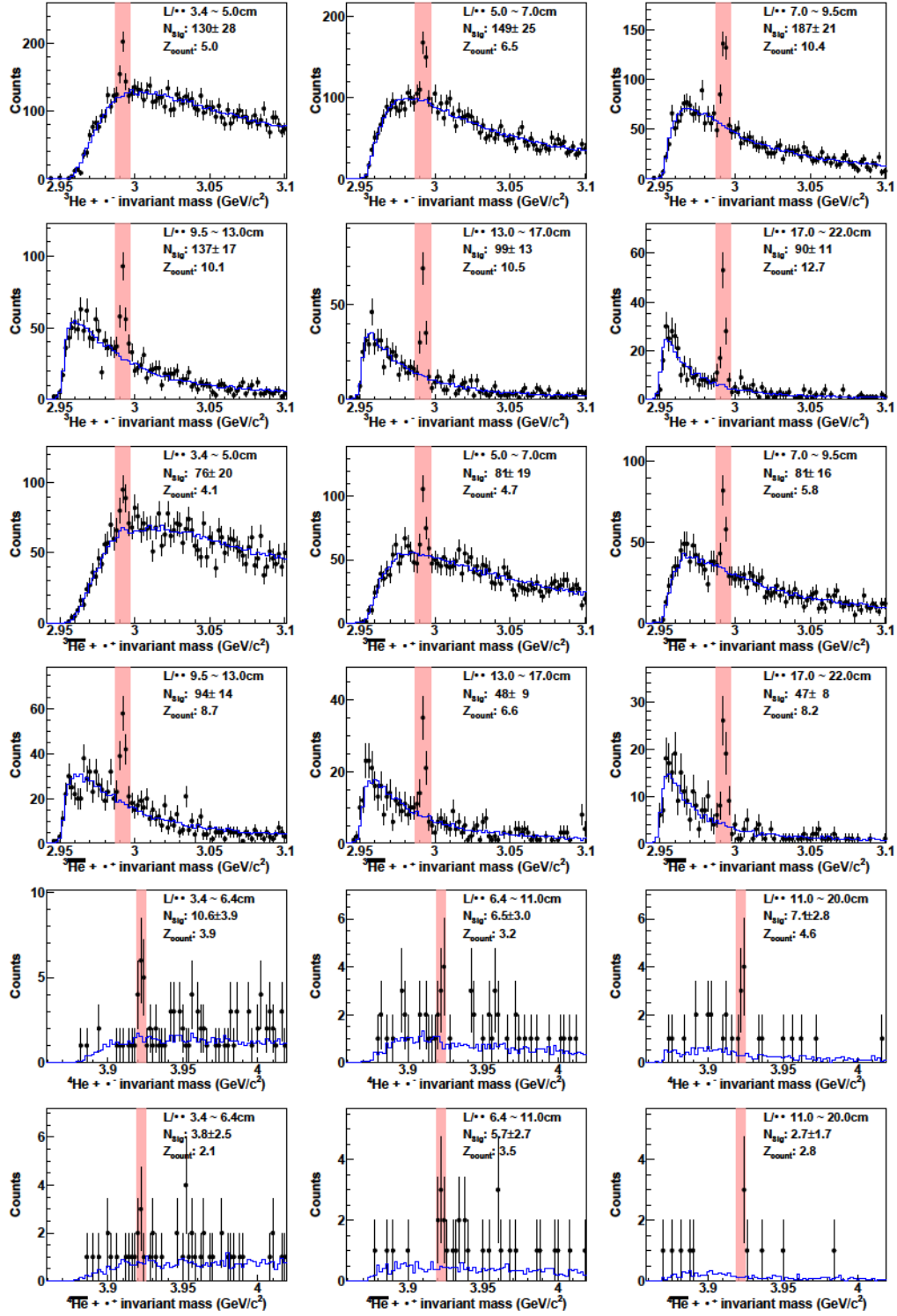
Figure 3: {}^3\text{H} , {}^3\bar{\text{H}} , {}^4\text{H} and {}^4\bar{\text{H}} candidate invariant-mass distributions in different L/\beta\gamma intervals.
