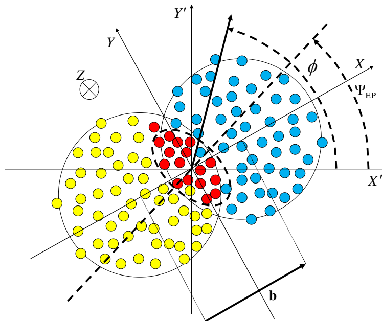
Figure 1. A schematic view of a non-central nucleus-nucleus collision in the transverse plane.
