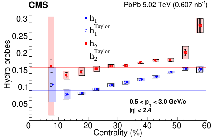
Figure 4. The h_1 = (v_2\{6\} - v_2\{8\})/(v_2\{4\} - v_2\{6\}) (closed blue circles) and the h_2 = (v_2\{8\} - v_2\{10\})/(v_2\{6\} - v_2\{8\}) (closed red squares) hydrodynamic probes as functions of centrality in PbPb collisions at \sqrt{s_{\text{NN}}} = 5.02 TeV. The distributions depicted with the open circles and squares represent the corresponding Taylor expansions given by h_1^{\text{Taylor}} and h_2^{\text{Taylor}} , respectively. The horizontal blue (red) line represents a constant value of 1/11 ( 3/19 ). The bars (the vertical sizes of the open boxes) denote the statistical (systematic) uncertainties. Points are plotted at the center of the respective centrality ranges.
