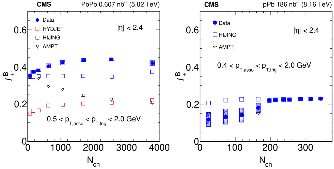
Figure 5. The integral of the balance functions ( I_{+-}^B ) in PbPb collisions at \sqrt{s_{NN}} = 5.02 TeV (left) and in pPb collisions at \sqrt{s_{NN}} = 8.16 TeV (right). The balancing partners fall within the specified pseudorapidity range ( |\eta| < 2.4 ) and have transverse momenta within the range of 0.5 < p_T < 2.0 GeV (for PbPb) and 0.4 < p_T < 2.0 GeV (for pPb). The statistical uncertainties in the data points are smaller than the marker size and rectangular boxes indicate the systematic uncertainties.
