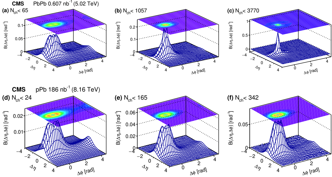
Figure 1. The balance function is shown in terms of \Delta\eta and \Delta\phi in PbPb collisions at \sqrt{s_{NN}} = 5.02 TeV (upper panels) and for p Pb collisions at 8.16 TeV (lower panels). From left to right, the results are shown for the lowest to highest multiplicity classes in PbPb and p Pb collisions. The trigger and associated particles in PbPb ( p Pb) collisions satisfy the condition 0.5(0.4) < p_{T,asso} < p_{T,trig} < 2.0 GeV.
