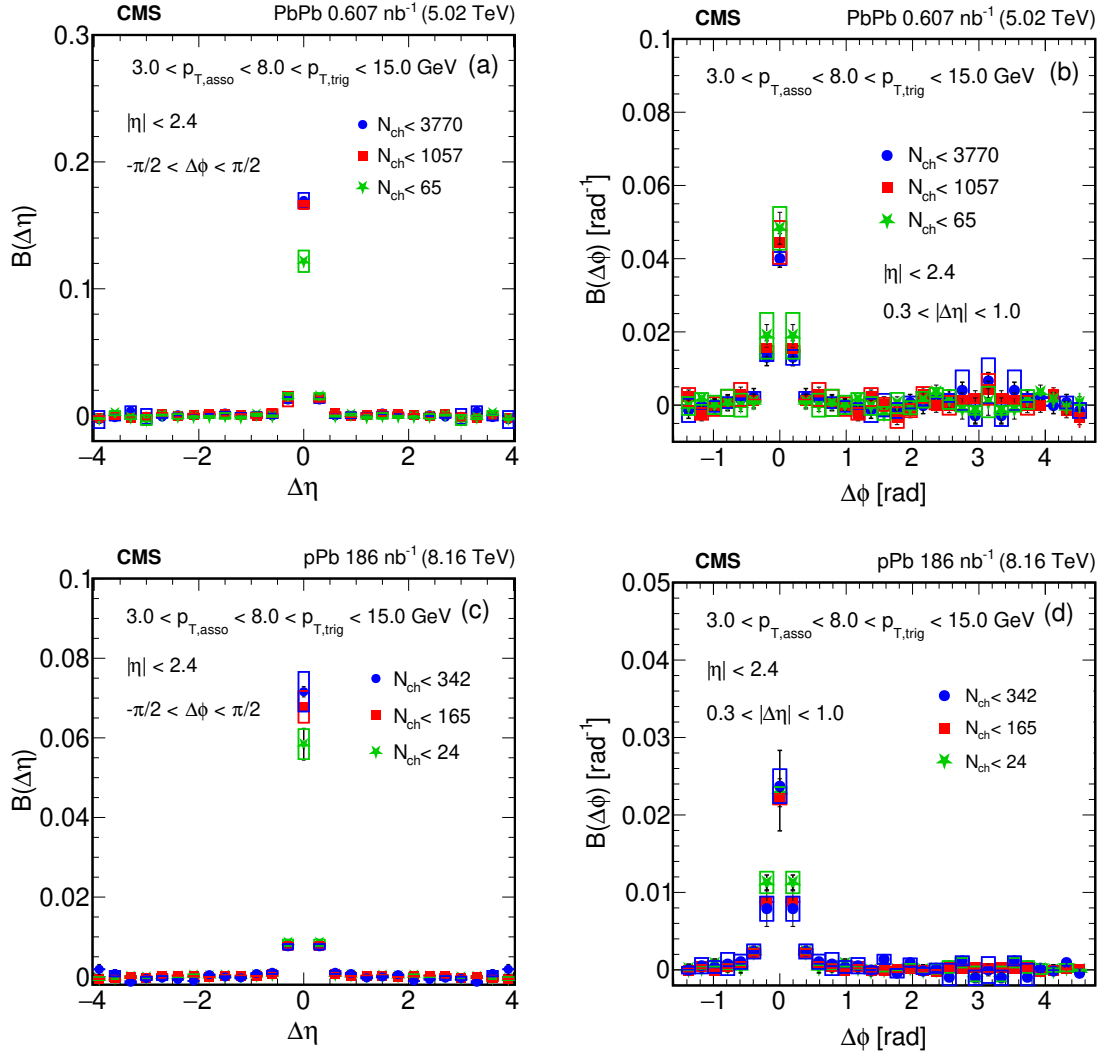
Figure 9. The projection of the balance function is presented for PbPb in \sqrt{s_{\text{NN}}} = 5.02 TeV (upper panels) and pPb in \sqrt{s_{\text{NN}}} = 8.16 TeV (lower panels) collisions as a function of \Delta\eta (left column) and \Delta\phi (right column), for 3.0 < p_{T,\text{asso}} < 8.0 < p_{T,\text{trig}} < 15.0 GeV ranges. The 1D projection is derived for \Delta\eta in near-side ( |\Delta\phi| < \pi/2 ) and \Delta\phi ( 0.3 < |\Delta\eta| < 1.0 ) regions.
