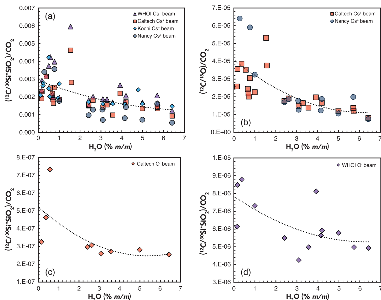
Figure 8. Effect of water on the (^{12}\text{C}/^{30}\text{Si}) \times \text{SiO}_2 / \text{CO}_2 and ^{12}\text{C}/^{18}\text{O} / \text{CO}_2 ratios measured by SIMS (i.e., the calibration line). The results of four SIMS sessions using a \text{Cs}^+ primary beam and two SIMS sessions using an \text{O}^- primary beam are reported. In all cases the glass water content seems to greatly reduce the ionisation efficiency of ^{12}\text{C} . Data used to generate the figure are reported in Table S9. Dotted lines are 2nd-order polynomial best fit to all data.
