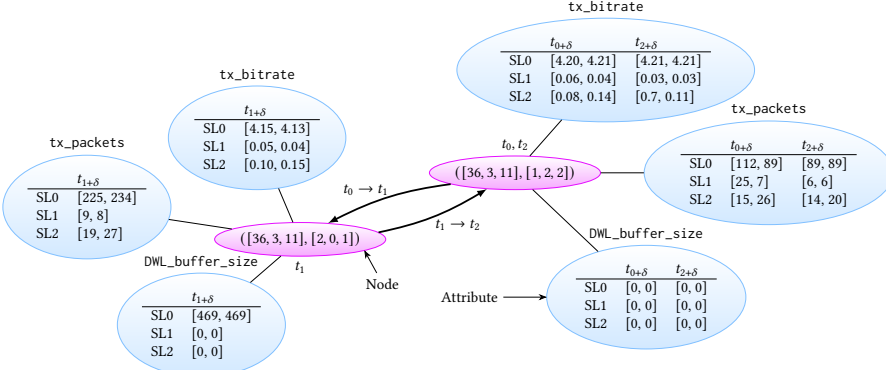
Fig. 11. Process of building the attributed graph during time steps t_0 , t_1 and t_2
