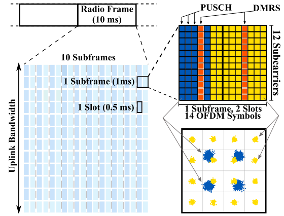
Fig. 1: Physical layer and Resource Grid of uplink data.
