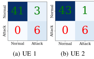
Fig. 10: The confusion matrices for two UEs demonstrates the ability of Det-RAN to detect the attacks.
