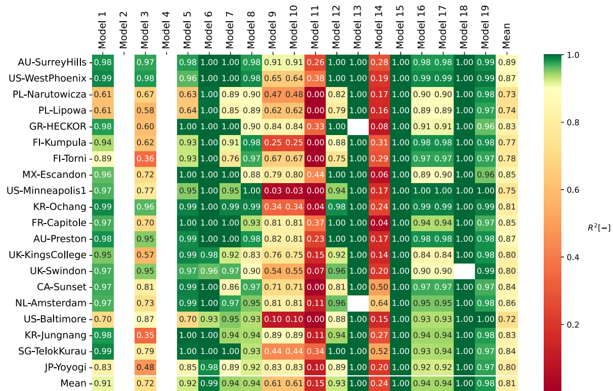
Figure 8. Coefficient of determination ( R^2 ) between (half-)hourly explicit (Equation 2) and implicit water storage change (Equation 1) by model and site. Green indicates the 0.9 I_{s,t} threshold (Table 1). Missing results are shown as white (i.e., cannot calculate explicit or implicit water storage change). Figure 9 may aid interpretation of R^2 values.
