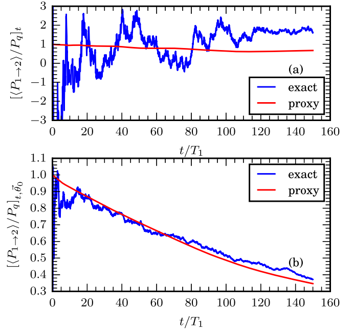
FIG. 8. (a) Time-averaged energy current calculated by numerical integration [\langle P_{1 \rightarrow 2} \rangle]_t / P_q (exact) and via the spin-lock fidelity, with AIM, [\hat{B} \cdot \langle \vec{\sigma} \rangle]_t (proxy) for a single initial phase \vec{\theta}_0 = (5.1545, 2.0452) . (b) Initial phase averaged (denoted as in Fig. 5) curves (1000 realizations) for the parameters: B_0 = 2 , A = 30 , T_1 = 300 in the skew BHZ model (2).
