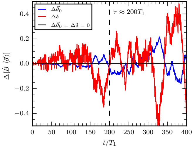
FIG. 7. Deviation in the spin-lock fidelity from the unperturbed set of initial conditions: B_0 = 2 , A = 30 , T_1 = 380 , \vec{\theta}_0 = (2.4, 5.3) (black line). The perturbation in initial phase is given by \vec{\theta}_0 = (2.401, 5.301) (blue line), with |\Delta\vec{\theta}_0| = O(10^{-3}) . The perturbation in adiabatic parameter is given by a change in T_1 (red line), with \Delta\delta = O(10^{-7}) .
