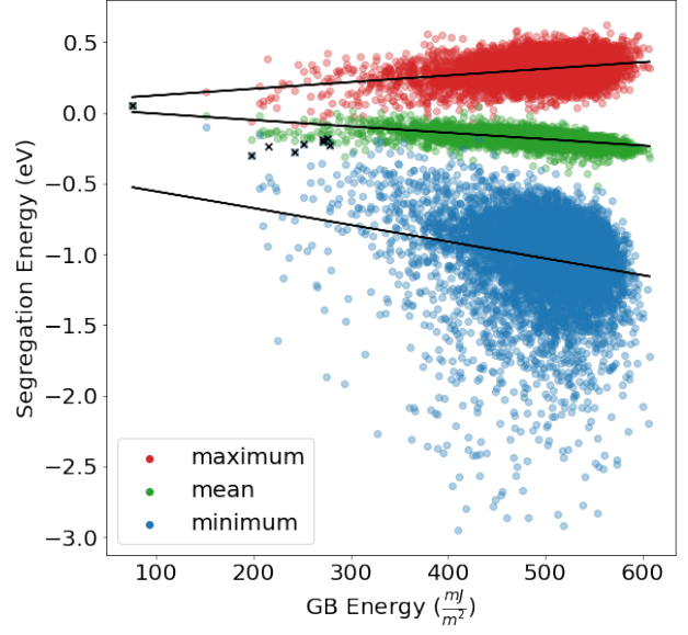
Figure 6: Maximum (red), mean (green), and minimum (blue) values of the segregation energy, E_{seg}^{Co_i} , spectrum for each GB vs. their GB interface energy, \gamma . Linear fits for each are shown in black. The mean segregation energy for the [111] symmetric twist GBs are shown with black “x” markings. The range of segregation energies increases with GB energy, and the mean segregation energy has an inverse relationship with increasing GB energy.
