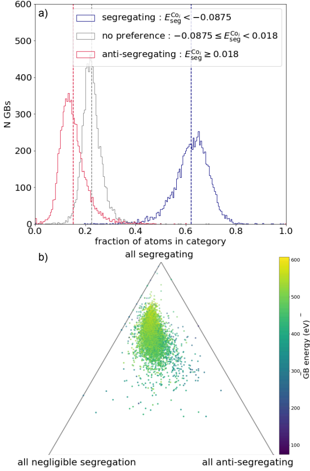
Figure 7: a) Histograms of f_{\text{seg}} (blue), f_{\text{anti}} (red), f_{\text{negl}} (grey) for GB atoms as determined by CSP. The mean of each histogram is marked with a dashed vertical line of a corresponding color. Bin size is 0.005 eV. b) Ternary scatter plot of the same data, colored by GB energy, \gamma . Since the sum of these values is 1 (i.e., f_{\text{seg}} + f_{\text{anti}} + f_{\text{negl}} = 1 ), they lie on a 2D plane in 3D space.
