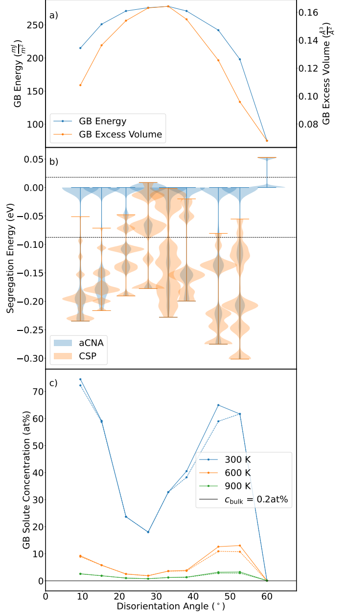
Figure 8: a) Plot of GB energy ( \frac{\text{mJ}}{\text{m}^2} ) and GB excess volume ( \frac{\text{\AA}^3}{\text{\AA}^2} ) as functions of disorientation angle ( ^\circ ) for the [111] symmetric twist GBs. b) Plot of the segregation energy (eV) spectra for GB atoms as determined by CSP (orange) and aCNA (blue) in the [111] symmetric twist GBs, against their disorientation angles. Aside from the perfect twin GB at 60° twist, their segregation energies are almost always negative, or favorable to segregation. The “negligible segregation” ( -0.0875 \text{ eV} \leq E_{\text{seg}}^{\text{Co}_i} < +0.018 \text{ eV} ) limits are shown with dotted black lines. c) Concentration of solute at the GB, c_{\text{GB}} (at.%), as a function of disorientation angle ( ^\circ ) and temperature for the [111] symmetric twist GBs, for CSP (solid) and aCNA (dotted). This is calculated using Equation 2. The bulk concentration, c_{\text{bulk}} = 0.2 \text{ at.}\% , is shown with a solid black line.
