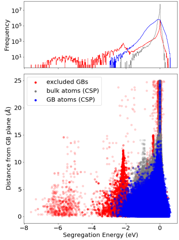
Figure 3: (Top) Histograms of segregation energy for GB atoms (blue), bulk atoms (gray), and atoms in GBs excluded due to invalid calculations (red). Bin width is 0.165 eV. A linear-scale histogram with the same data is included as Supplemental Figure S8 to show how low segregation energies contribute negligibly to the distribution. (Bottom) Distance from the GB plane in Å as a function of segregation energy, ( E_{\text{seg}}^{\text{Co}_i} ). In the GB construction simulations, the GB plane is initialized at z = 0 Å and is allowed to shift as the simulation cell relaxes, however, this distance is calculated as a distance from z = 0 Å. The non-converged and low energy GBs that were removed from analysis as described in Sections 3.1.1 and 3.1.2 are shown in red, the bulk FCC atoms as determined by a CSP cutoff of 0.1 are shown in grey, and the non-bulk GB atoms are shown in blue. The distribution decays to 0 eV as the distance from the GB increases (with the exception of the excluded GBs, shown in red), as predicted in [62, 63].
