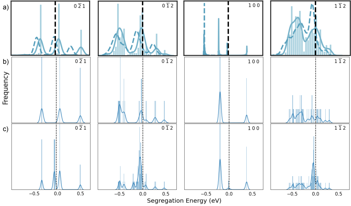
Figure 4: Segregation energy distributions of the shared \Sigma GBs between the a) Huber dataset from [31] (bin width 0.04 eV) and the b/c) Homer dataset (bin width 0.01 eV). a) has two fit lines: a KDE fit to the data (solid) and a model fit discussed in [31] (dashed). b) includes the non-bulk atoms from this work as determined by aCNA (the same method of FCC atom removal as is used in [31]). c) includes the non-bulk atoms from this work as determined by CSP. The Huber dataset in a) is reproduced from [31] and relabeled according to the Homer dataset labelling conventions [52].
