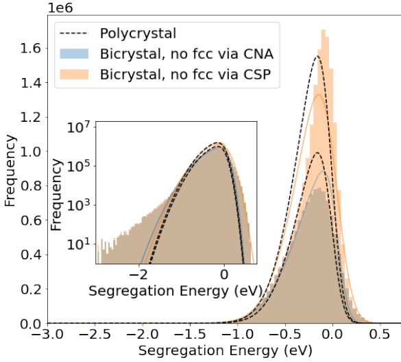
Figure 5: The spectrum of segregation energies aggregated from all GBs simulated in this work, with all bulk atoms removed via aCNA (blue) and via CSP (orange), with fit lines for their respective skew-normal distributions in the form of Equation 3 in their respective colors. The dashed black lines are the polycrystal spectrum from Wagih et al. in [27], scaled to both of this work’s distributions. Inset are the same spectra on a logarithmic scale. Statistics for each skew-normal distribution are given in Table 1. The spectrum of all atoms (including bulk atoms) is shown in Supplemental Figure S12. Bin width is 0.0412 eV.
