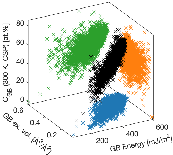
Figure 11: Concentration of solute at the GB, c_{GB} , as a function of GB excess volume and GB energy. The following are projected onto their corresponding planes: c_{GB} vs. GB energy (green), c_{GB} vs. GB excess volume (orange), and GB excess volume vs. GB energy (blue).
