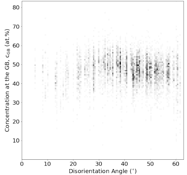
Figure 10: Disorientation angle vs. concentration in the GB, c_{GB} at 300 K using CSP for GB atom selection.
