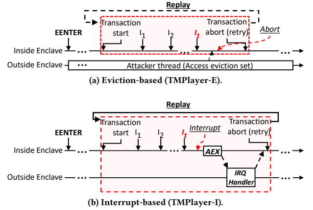
Figure 4: TMPlayer-based instruction replay.
