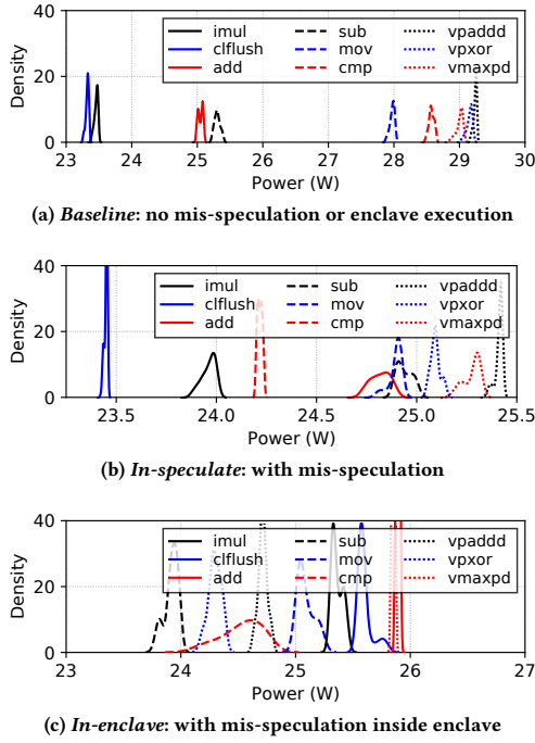
Figure 6: Power signature of representative instructions in different execution environments ( \mu Code 0xF0).
