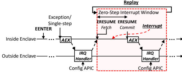
Figure 1: Timeline for timer interrupt-based replay.
