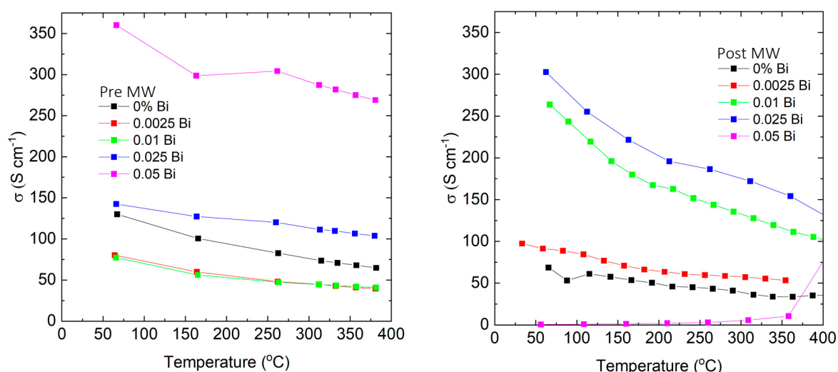
Figure 3. Electrical conductivity vs. temperature for samples quenched from melt before (left) and the same samples after (right) annealing in a single-mode microwave cavity.
