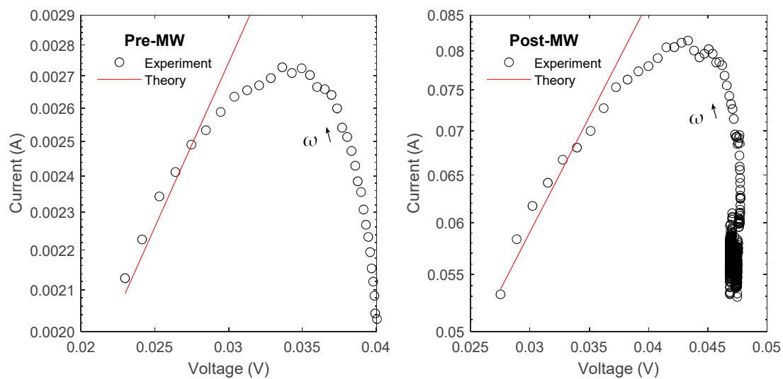
Figure 13. The Richardson equation was adapted to incorporate the applied voltage and fitted to the experimental data by adjusting the energy barrier height relative to the bulk Fermi level.
