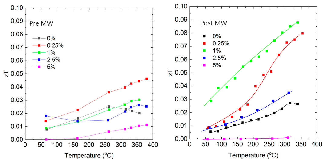
Figure 15. Dimensionless figure of merit ( zT ) vs. temperature for samples quenched from melt ( left ) and after microwave annealing ( right ). Solid lines are guides for the eyes.
