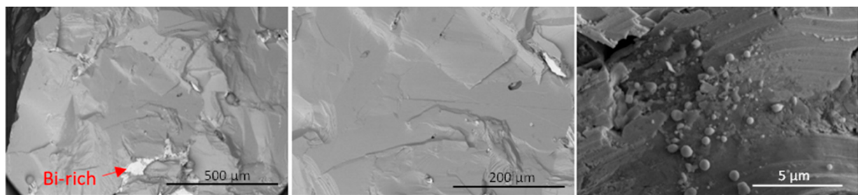
Figure 11. Backscattered electron images of GaSbBi 0.05 :Te fracture surface, exhibiting numerous cracks crossing the fracture plane. These cracks potentially contribute to the remarkably low electrical conductivity observed in this material after microwave treatment. Localized melting events can lead to substantial residual strains due to the volume expansion upon resolidification, which may explain the observed conductivity reduction.
