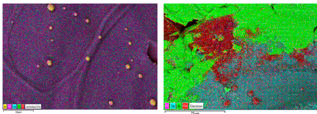
Figure 12. EDS layered maps revealing the presence of Bi-rich regions in the GaSbBi 0.0025 (left) and GaSbBi 0.05 (right) samples. These Bi-rich regions correspond to the bright particles observed in the backscattered SEM images.
