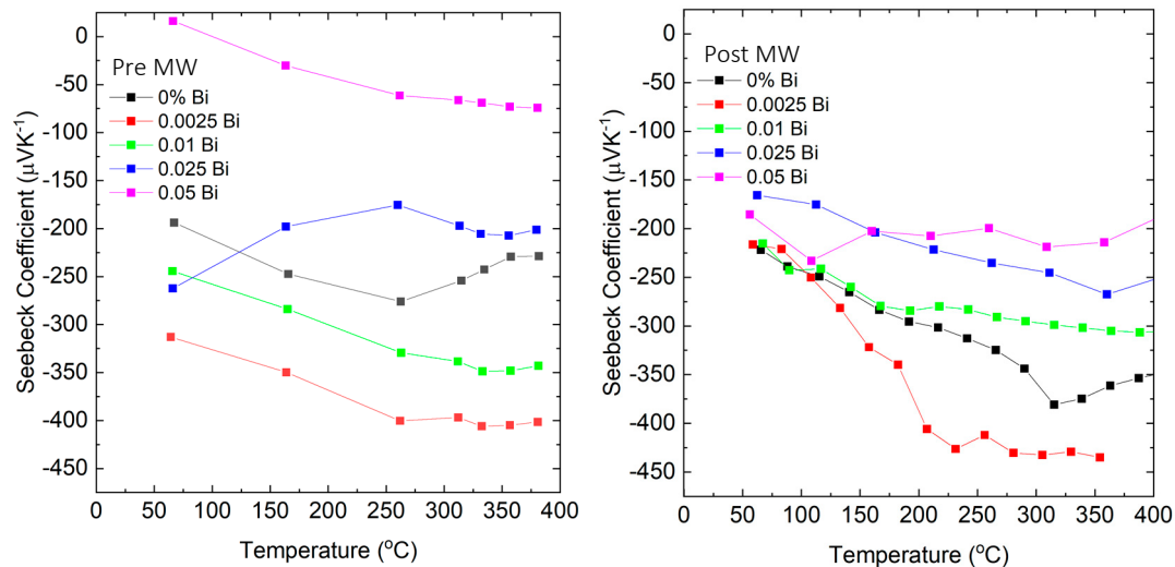
Figure 4. Seebeck coefficient vs. temperature for samples quenched from melt before ( left ) and the same samples after ( right ) annealing in a single-mode microwave cavity.
