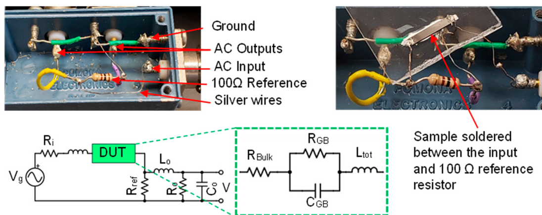
Figure 6. Circuit diagram of the AC impedance measurement setup and a model equivalent circuit representing a polycrystalline semiconductor sample with an energy barrier that permits leakage due to finite resistance in the charge-depleted regions at compensating-type grain boundaries. The inductor illustrates two phenomena: the inductance of the sample and the reduced capacitance of the energy barrier at high frequencies.
