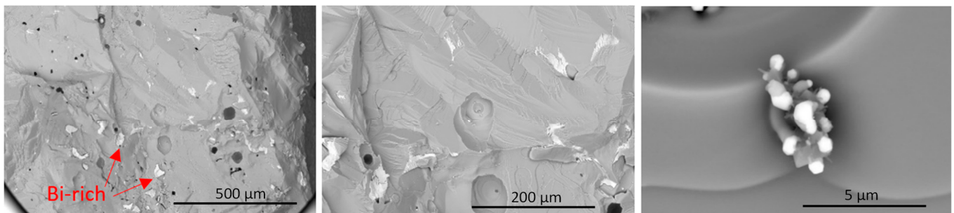
Figure 10. Backscattered electron images of GaSbBi 0.0025 :Te fracture surface, revealing bright regions indicating the presence of Bi-rich areas due to atomic number contrast from scattering.
