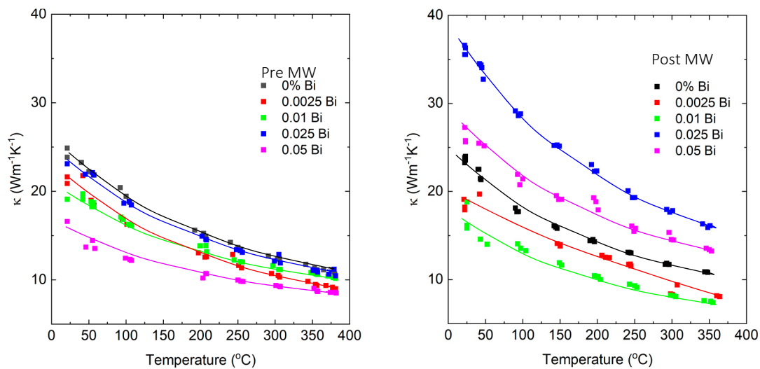
Figure 14. Thermal conductivity vs. temperature for samples quenched from melt ( left ) and after microwave annealing ( right ).
