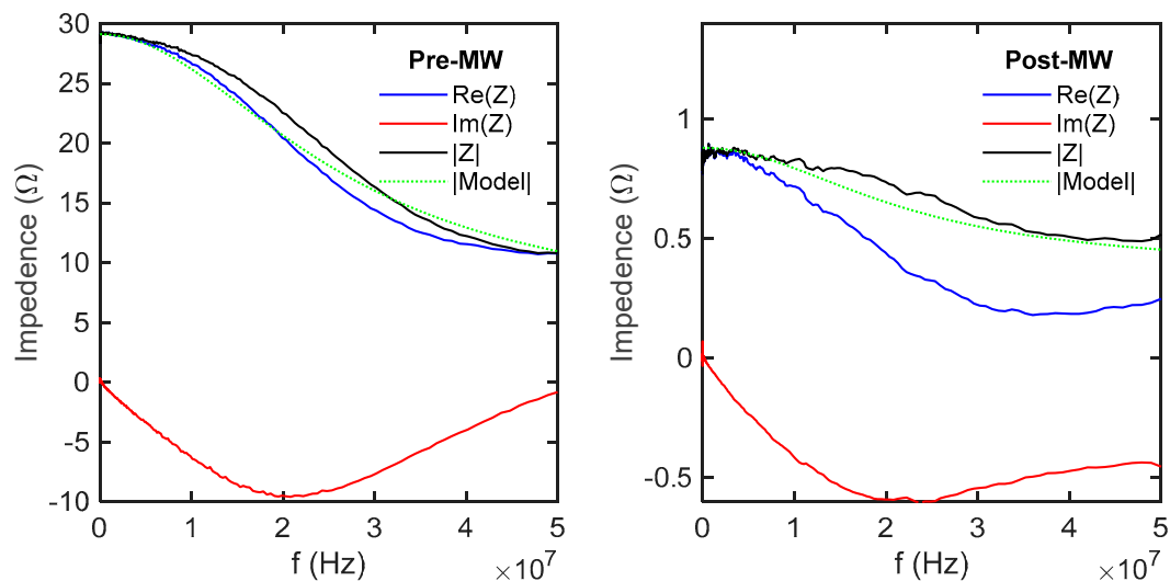
Figure 8. The impedance of the sample was determined by measuring the voltage across a reference circuit while sweeping the frequency. The known voltage on the reference circuit enabled the determination of the current in the sample, allowing for the calculation of the impedance.
