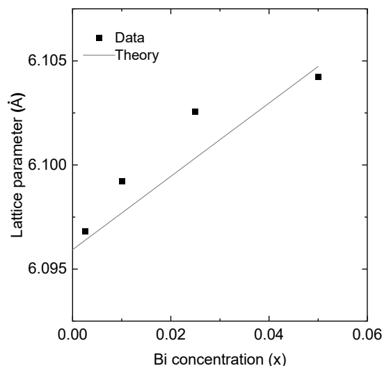
Figure 2. Lattice parameter determination based on the measured position of the (111) peak.
