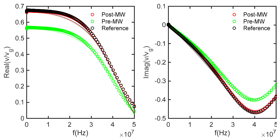
Figure 7. The reference curve is fitted by holding R_i , R_o , R_{\text{ref}} , and V_g constant while varying C_o , L_o , and L_i . Subsequently, preliminary values for R_{\text{bulk}} , R_{\text{GB}} , C_{\text{GB}} , and L_{\text{tot}} were also successfully estimated.
