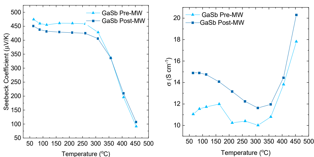
Figure 5. Comparison of Seebeck coefficient and electrical conductivity for a commercially-produced GaSb powder post densification via spark plasma sintering (SPS) and following subsequent microwave treatment.
