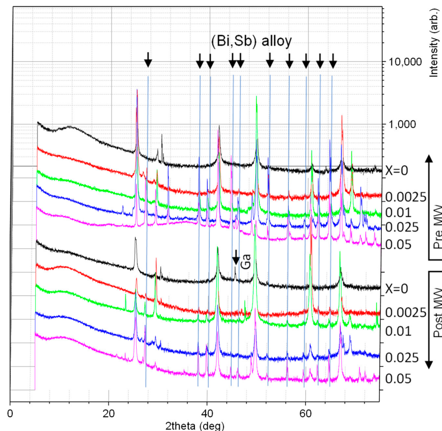
Figure 1. X-ray Diffraction data, with peak positions labeled for Ga and \text{Bi}_{0.84}\text{Sb}_{0.16} alloys as identified using PDXL2 software (version 2.9.1.0). Peaks not labeled correspond to those expected in GaSb.
