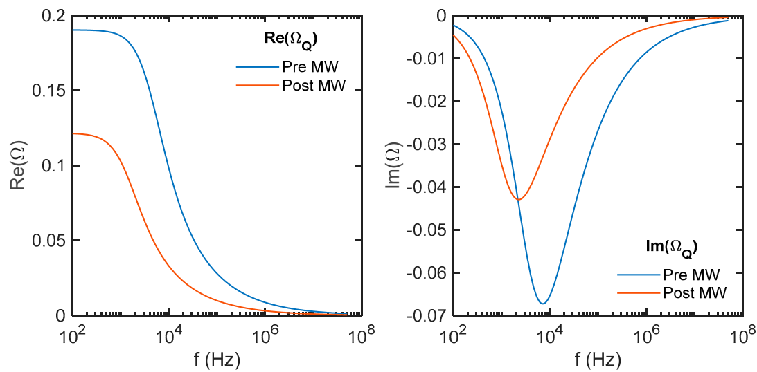
Figure 9. The calculated impedance resulting from the heat transferred within the sample through the Peltier effect, followed by its conduction into the glass slide to which the samples are mounted.
