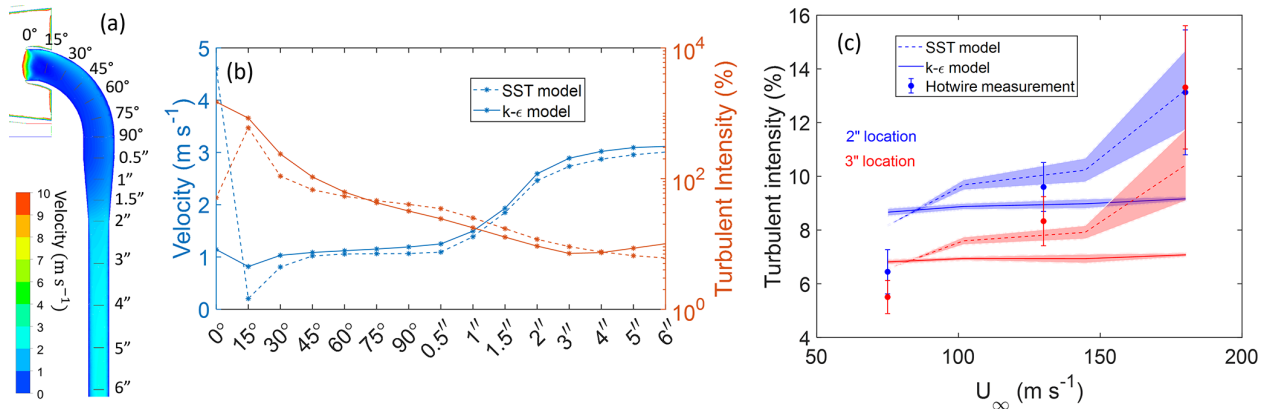
Figure 4. Simulation results inside the sampling tube for ground-level conditions in Table 1 ( 180 \text{ m s}^{-1} , a 25 mm restrictor, 3 % freestream turbulence, 3° angle of attack). (a) Contour of velocity magnitudes in the center plane of the sampling tube, with different locations relevant for (b) labeled. (b) Surface-weighted average of turbulent intensities and velocities along the length of the sampling tube. (c) Comparisons of turbulent intensity measured and simulated inside the sampling tube. The simulated sampling flow rate is Q_{\text{sampling}} = \sim 19 \text{ SLPM} ; the shading reflects varying TI_{\infty} from 0.5 % to 3 % in the models. The hot-wire measurements show average values for a 15 and 20 SLPM sampling flow rate; error bars represent the range of measurements at the two sampling flow rates.
