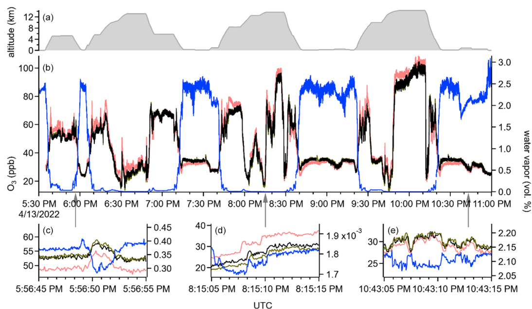
Figure 2. Time stamp synchronization based on the \text{H}_2\text{O} and \text{O}_3 time series. VCSEL data are shown in blue, Fast \text{O}_3 data in salmon, FAIRO 1 in black, and FAIRO 2 in dark olive. All traces are shown at the native instrument resolution (25 Hz for VCSEL, 12.5 Hz for the FAIROs, and 10 Hz for Fast \text{O}_3 ). (a) Altitude time series. (b) Time series for the entire flight. (c–e) Zoomed-in views of cross-covariance events, with gray arrows pointing to exact times.
