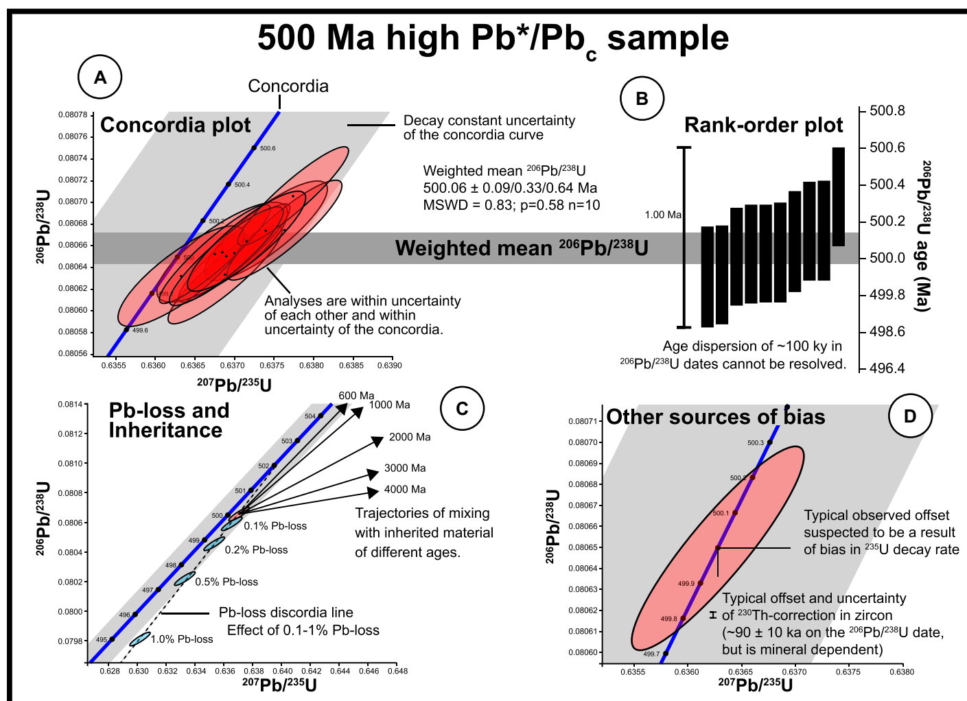
Figure 2. Impact of different types of system complexity on precise U-Pb dates in Wetherill concordia plots and age ranked plots for analyses of a 500 Ma high Pb*/Pb c sample. (A) Concordia plot of high Pb*/Pb c analyses situated within concordia curve uncertainty. Excellent reproducibility (mean square of weighted deviates [MSWD] = 0.83) allows for calculation of a weighted mean age. (B) Representation of the ^{206}\text{Pb}/^{238}\text{U} dates in a rank order plot; individual dates are statistically equivalent and do not resolve a hypothetical 100 k.y. duration of mineral growth. (C) High Pb*/Pb c analyses delineating a lead-loss trend that becomes visible at >0.5% Pb-loss at the chosen uncertainty of individual dates. Graph also shows different mixing trajectories toward xenocrystic/inherited components diverging from the concordia, leading to discordance as a function of the age of the xenocrystic component as well as of the analytical precision. (D) Effect of ^{230}\text{Th} disequilibrium on a 500 Ma zircon with a high Pb*/Pb c level as well as on suspected \lambda_{235\text{U}} inaccuracy (see text for discussion). Expected shifts in the concordia space stay within the analytical uncertainty ellipse and the decay constant uncertainty band of the concordia, respectively. Amount of ^{230}\text{Th} disequilibrium and its uncertainty will be different for different minerals; e.g., see Parrish (1990).
