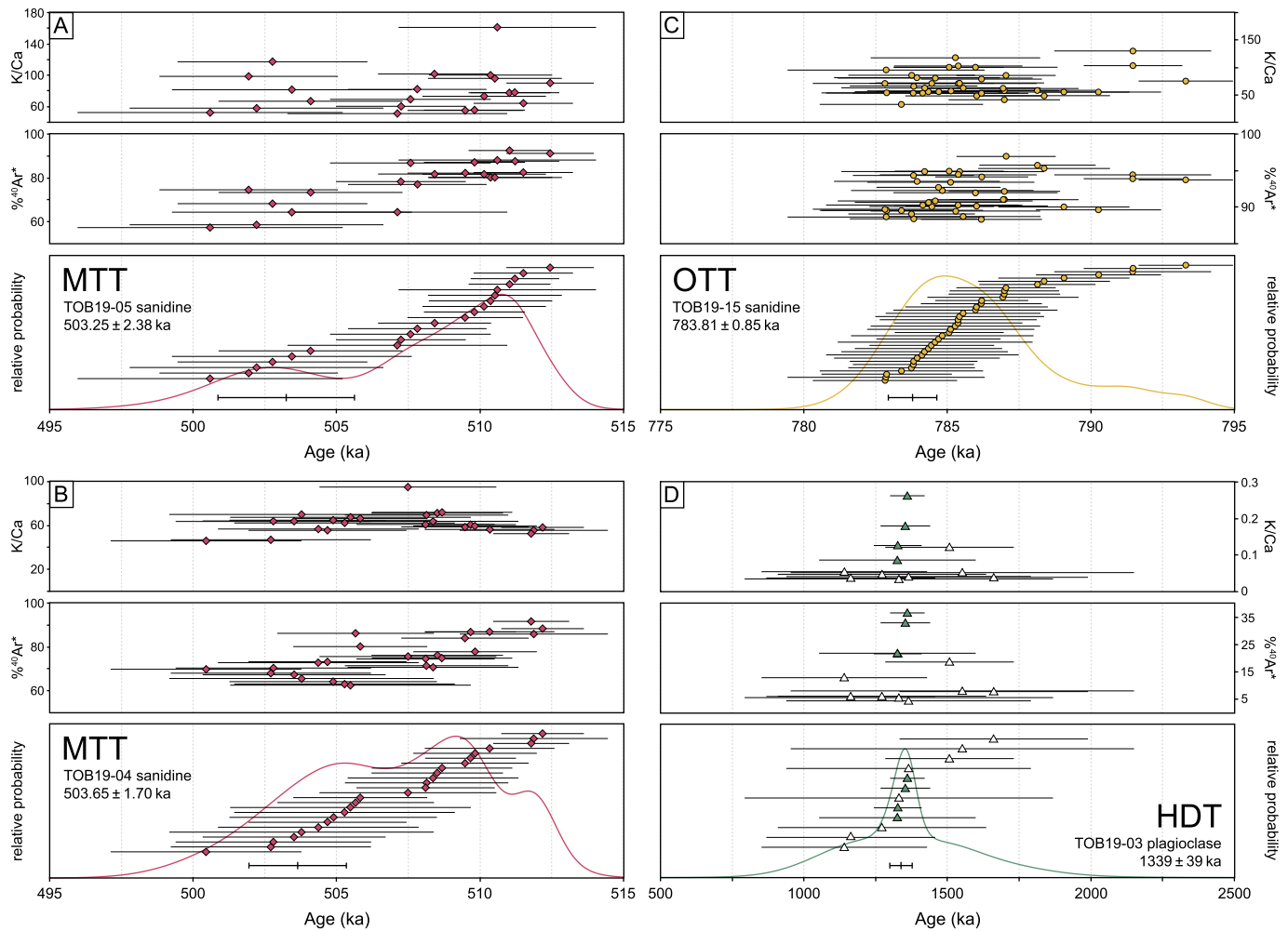
Fig. 3. ^{40}\text{Ar}/^{39}\text{Ar} feldspar geochronology of the Toba tuffs: MTT (A, B), OTT (C), and HDT (D). %Ar* – percent radiogenic Ar. Eruption ages were estimated using the Bayesian model of Keller et al. (2018) with an exponential prior distribution, using all data (MTT, OTT) or only data with >20% Ar* (HDT). The two MTT samples are combined to calculate a best-estimate MTT age in Table 1. All error bars represent 2\sigma analytical uncertainties.
