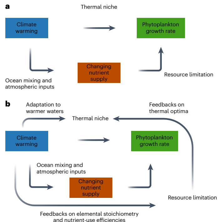
Fig. 5 | Developing improved ESMs of ocean warming and nutrient interactions.
