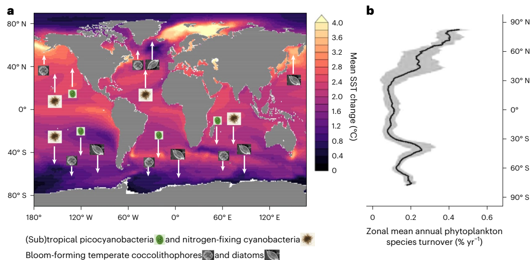
Fig. 1 | Projected poleward shifts in distributions of biogeochastically important phytoplankton functional groups with extreme warming.
