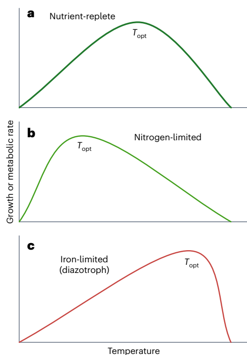
Fig. 2 | Idealized temperature response curves for growth and metabolic rates relative to nutrient availability in phytoplankton. a–c. Typical curves for nutrient-replete cells 51,56,62 ( a ), nitrogen-limited cells 56 ( b ) and iron-limited cells (specifically for the diazotrophic cyanobacterium Trichodesmium ; c ) 62 . Decreasing trends in T_{opt} under N limitation and increasing trends in T_{opt} under Fe limitation in the diazotroph are depicted.
