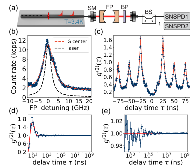
Fig. 3 | Quantum coherence of G center emission. a Emission from the G center is collected through a single mode (SM) fiber and analyzed with a tunable Fabry Perot (FP) cavity. BP: Bandpass filter, BS: beamsplitter. b Measured emission linewidth (red fit): 6.2(1) GHz, FP linewidth (black, using reference laser): 3.4(1) GHz. Calculated G center linewidth after deconvolving the FP response: 2.8(1) GHz. c Normalized intensity correlations at the detectors g^{(2)}(\tau) show single-photon emission g^{(2)}(0) = 0.15(2) < 0.5 . d, e Long term intensity correlations under continuous wave excitation show stable single-photon emission. c–e Error bars represent Poissonian noise, and the error of reported values is the error of the fits.
