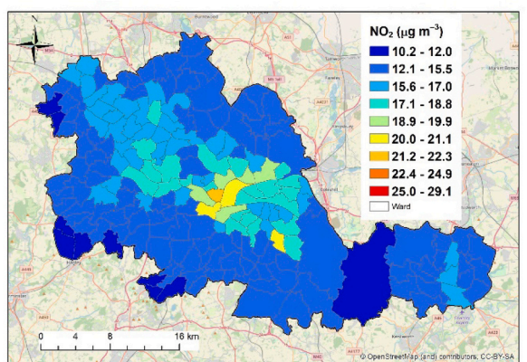
Fig. 8. Annual air quality map of NO 2 (in \mu\text{g m}^{-3} ) at the ward level for (a) Case 2019 BAU, and percentage change (reduction in %) of NO 2 for (b) Case Re0.1, (c) Case Re0.3, (d) Case Re0.5, (e) Case Re0.7, and (f) Case Re0.9, relative to Case 2019 BAU.
