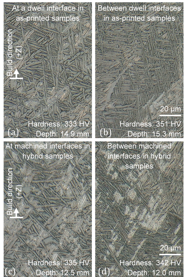
Fig. 14. Grain morphology at and between interfaces in the as-printed (a, b) and hybrid (c, d) samples.
