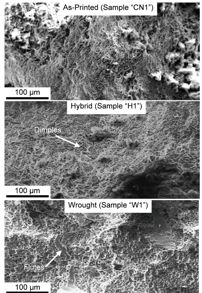
Fig. 19. Fractography of samples after tensile testing.
