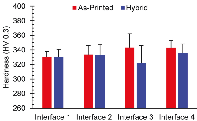
Fig. 13. Region 3 microhardness at dwell and machined interfaces identified in Fig. 11(a).
