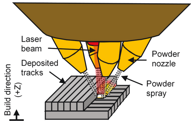
Fig. 3. Schematic of DED using LENS.
