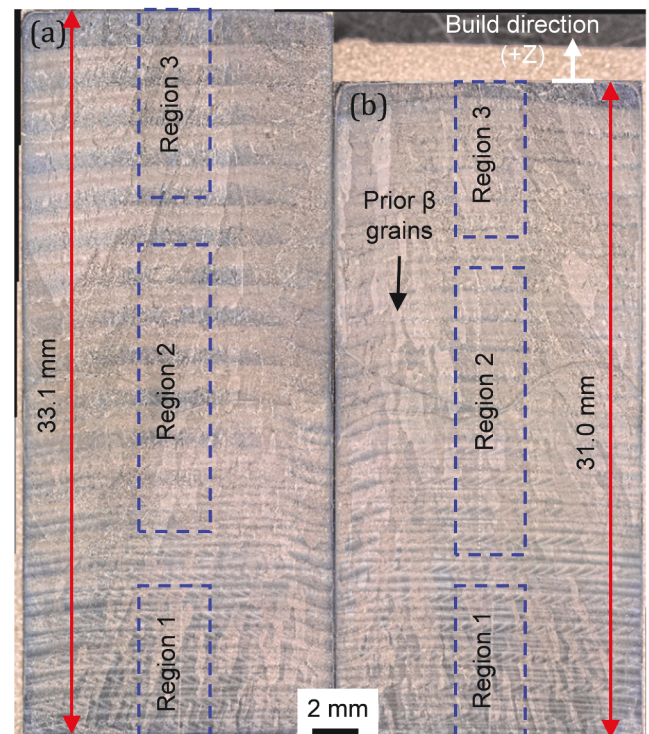
Fig. 5. (a) As-printed and (b) hybrid samples showing prior \beta -grain growth across multiple layers.
