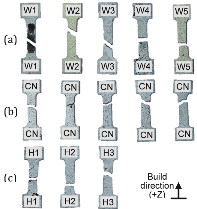
Fig. 18. Fracture patterns for (a) wrought, (b) as-printed, and (c) hybrid Ti-6Al-4 V.
