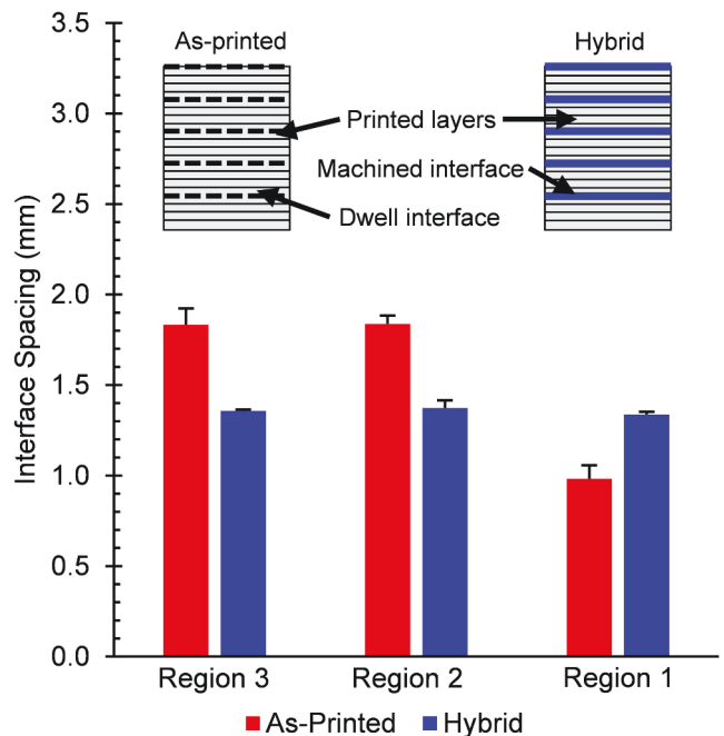
Fig. 15. Interface spacing in printed Ti-6Al-4 V from microhardness characterization.
