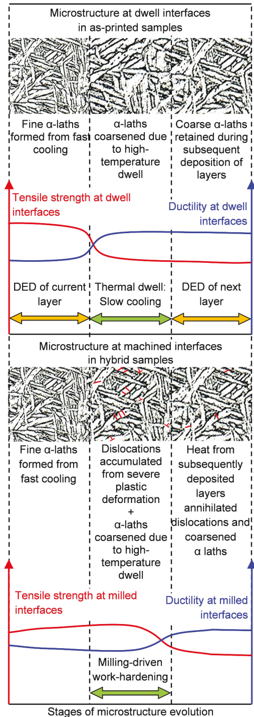
Fig. 20. Proposed mechanism for Ti-6Al-4 V microstructure formation from interlayer milling (adapted from [42,45,46]).
