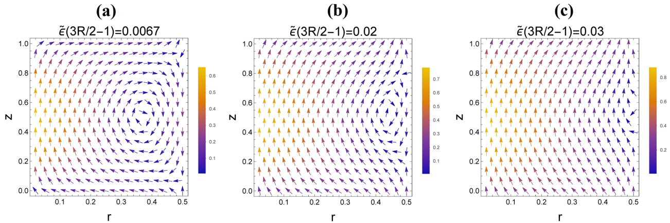
Figure 4. The slow-manifold radial and vertical velocity components for the rigid particles, plotted in the r – z plane for (a) \tilde{\varepsilon}\left(\frac{3R}{2}-1\right) = 0.0067 , (b) \tilde{\varepsilon}\left(\frac{3R}{2}-1\right) = 0.02 , and (c) \tilde{\varepsilon}\left(\frac{3R}{2}-1\right) = 0.03 . Other parameters are as listed for Experiment 1a in Table 1.
