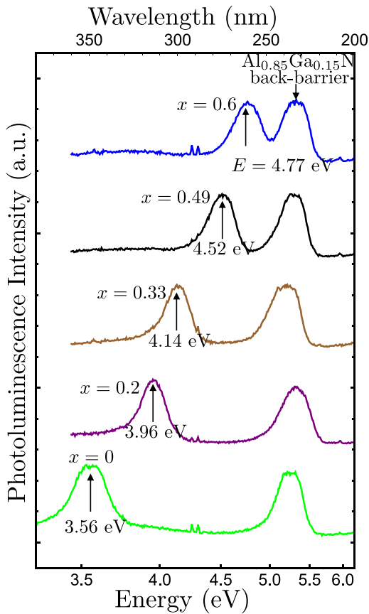
FIG. 2. Photoluminescence spectra of N-polar \text{Al}_x\text{Ga}_{1-x}\text{N}/\text{Al}_{0.85}\text{Ga}_{0.15}\text{N} heterostructures with varying Al composition x of the top AlGa channel layer at T = 300 K, showing photon emission from all the samples.
