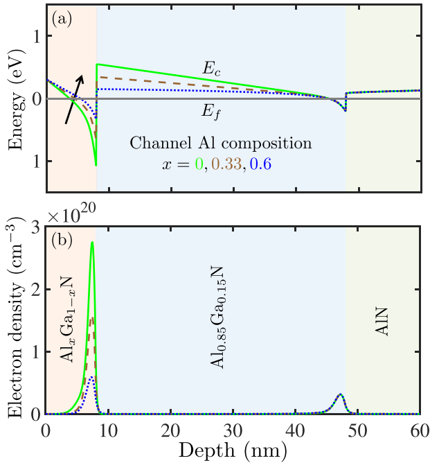
FIG. 3. (a) Simulated energy band diagrams for three different Al compositions x = 0 (green), 0.33 (brown), and 0.6 (blue) with a surface barrier height q\phi_B \sim 0.3 eV. (b) Simulated electron densities confirm the presence of high-density 2DEGs at \text{Al}_x\text{Ga}_{1-x}\text{N}/\text{Al}_{0.85}\text{Ga}_{0.15}\text{N} interfaces. The secondary channel at the bottom interface does not show measurable conductivity. 19
