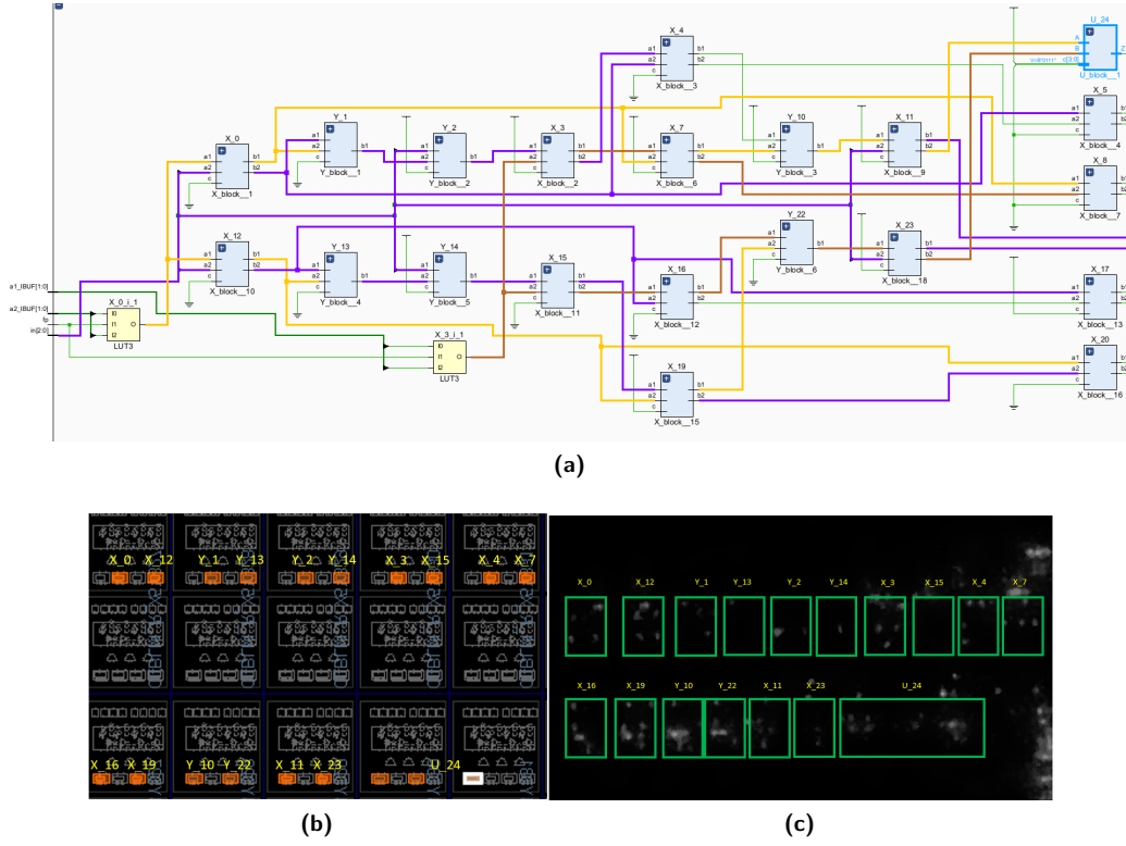
Figure 12: ISCAS85 - C17 placement of the sub-circuit connected to the first U-blocks (marked in blue at the top right corner): (a) shows the paths for 2 inputs connected to the U-block (orange and purple paths); (b) illustrates the placement of the circuit using the Vivado design suite, implementation view; (c) depicts the photon emission results of the LUTs in the circuit for the input pattern 6 (see Table 1).
