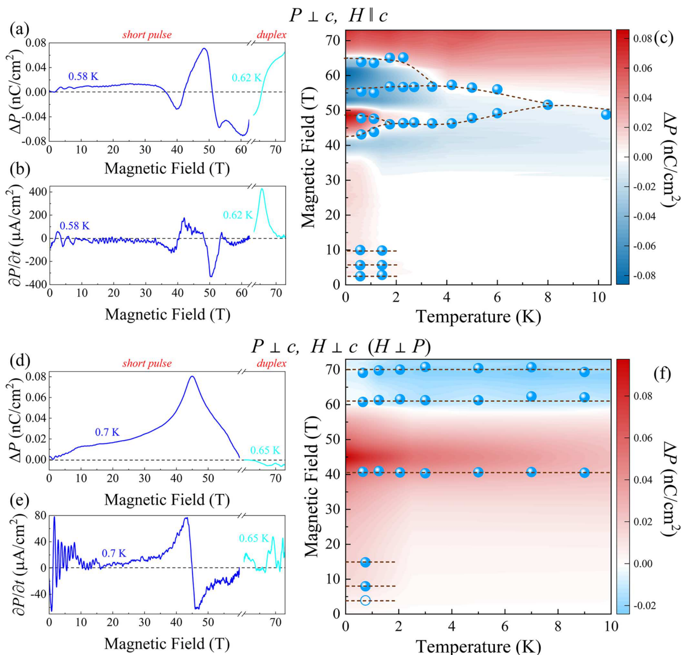
Figure 2. Magneto-electric response of [\text{Cu}(\text{pym})(\text{H}_2\text{O})_4]\text{SiF}_6 \cdot \text{H}_2\text{O} in the P \perp c, H \parallel c and P \perp c, H \perp c ( H \perp P ) configurations. (a, d) Change in the electric polarization ( \Delta P ) as a function of magnetic field for the P \perp c, H \parallel c and P \perp c, H \perp c ( H \perp P ) configurations, respectively. Data from the short pulse magnet is shown in navy blue, while data from the duplex magnet is shown in cyan. (b, e) Magneto-electric current vs magnetic field in the indicated configurations. (c, f) H - T phase diagrams of [\text{Cu}(\text{pym})(\text{H}_2\text{O})_4]\text{SiF}_6 \cdot \text{H}_2\text{O} in two different configurations. The solid blue symbols indicate phase boundaries at various measurement temperatures. The open symbol represents a point with some uncertainty. Error bars are on the order of the symbol size, and the dashed lines guide the eye.
