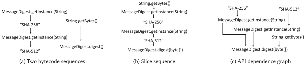
Fig. 1. API and constant sequences from bytecode, program slices, and API dependency graphs.
