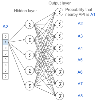
(b) Workflow of training token-level embedding using skip-gram.
