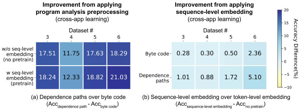
Fig. 10. The accuracy differences of sequence-level embedding, and program analysis preprocessing one new App sets 3, 4, 5, 6. (a) shows the accuracy difference of program analysis preprocessing (program slicing + API dependence graph construction), which are the accuracies achieved on API dependence paths minus the accuracies achieved on bytecode sequences. (b) is the accuracy difference of sequence-level embedding, which is the accuracies achieved with sequence-level embedding minus the accuracies achieved without sequence-level embedding.
