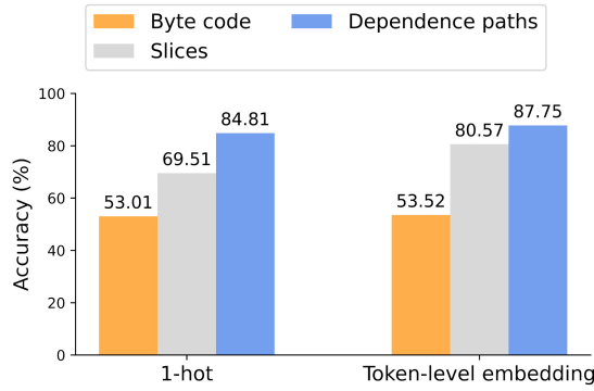
Fig. 3. Comparison of accuracy of with and without token-level embedding and applying different program analysis preprocessing (based on LSTM-128). The group on the left are results without embedding. The group on the right are results with token-level embedding. Applying token-level embedding improves the model performance in all three cases. The three colors represent three different program analysis approaches. With or without embedding, the dependence path outperforms the other two strategies and the slice outperforms bytecode. Compared to applying embedding, program analysis preprocessing boosts performance more.
