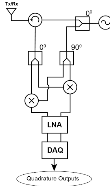
Fig. 1. Block diagram of a quadrature architecture Doppler radar measurement system.
