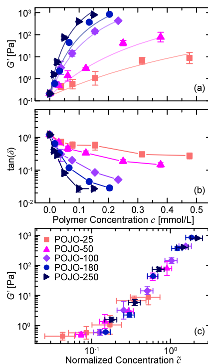
Figure 3. (a) Storage modulus G' and (b) loss tangent \tan(\delta) as a function of polymer concentration c at \omega = 10 rad s ^{-1} . Curves in (a) are fits to eq 1 and in (b) are guides to the eye. (c) Storage modulus G' as a function of normalized polymer concentration \tilde{c} = mc . Error bars in y are one log-normal standard deviation, and error bars in x are 95% confidence intervals on the fitting parameter m .
