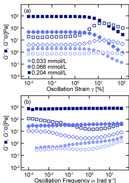
Figure 2. Storage modulus G' (closed) and loss modulus G'' (open) as a function of (a) strain amplitude \gamma at a fixed frequency \omega = 10 rad s ^{-1} and (b) as a function of frequency \omega at a fixed amplitude \gamma = 0.3\% for emulsions containing POJO-180 of varying concentrations c .
