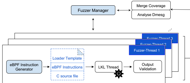
Figure 2: System overview of the lightweight Linux eBPF Fuzzer.
