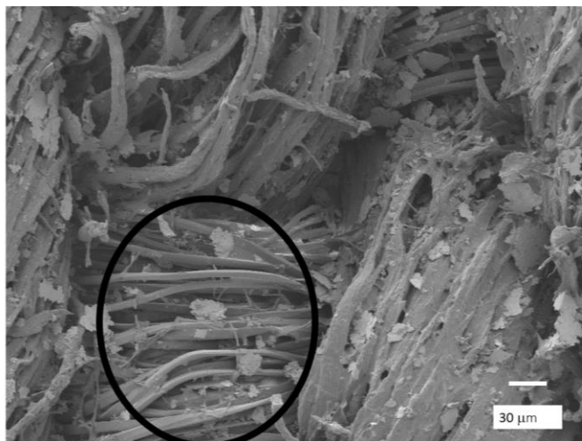
Fig. 5. Higher magnification image of sample R-W after 77 days. Undegraded polyester fibers circled.
