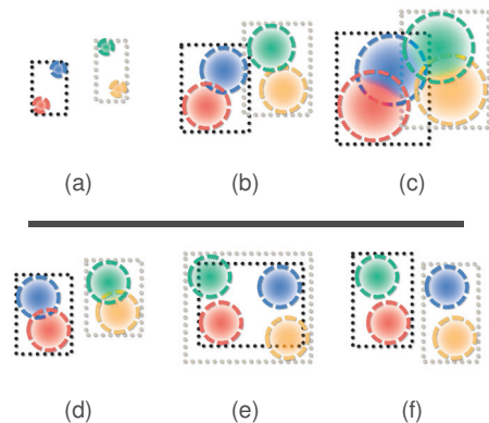
Fig. 5: Illustrations of bounding boxes over a dynamic scene: On the top figure we see particles (a) with expanding radii (b) that can be handled by tree refitting (c); on the bottom, we see particles with changing positions (d) that may create suboptimally overlapping bounding boxes (denoted with dotted lines) (e) hence requiring rebuilds (f).
