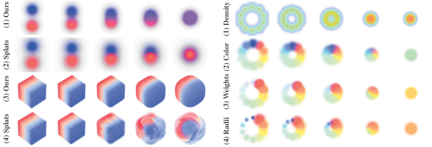
(a) Attribute-Aware Radial Basis Functions (1) use a world-space color blending, overcoming compositing limitations of prior splatting methods (2). Since our approach uses a stackless traversal over overlapping points (3), we safely avoid stack overflow issues exhibited by prior work [15] when ray-particle overlap is large (4).
