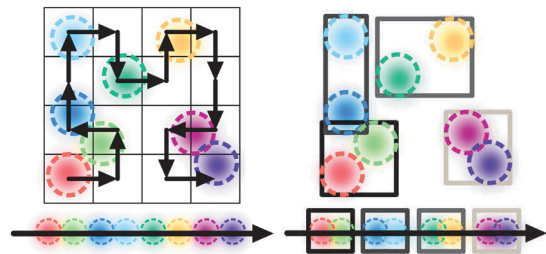
Fig. 6: Sorting the particle along a Hilbert curve to quickly and efficiently create spatially coherent clusters (denoted in solid lines).
