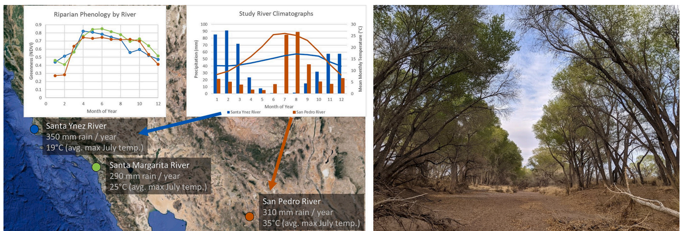
Fig. 2. Geographic, climatic, and habitat context for this study. At left: focal sites from the American Southwest with differences in climate (climatograph inset; lines are mean temperature and bars are precipitation) but similar riparian woodland composition and seasonality (phenology inset). Colors in the inset graphs correspond to the three focal sites – blue for VSFB, green for MCBCP, and orange for FH. At right: representative example of Fremont cottonwood ( Populus fremontii ) gallery woodland along an intermittent reach of the San Pedro River near FH. Climatographs are based on areal averages of long-term normal PRISM data across each study extent (PRISM Climate Group, 2014). (For interpretation of the references to colour in this figure legend, the reader is referred to the web version of this article.)
