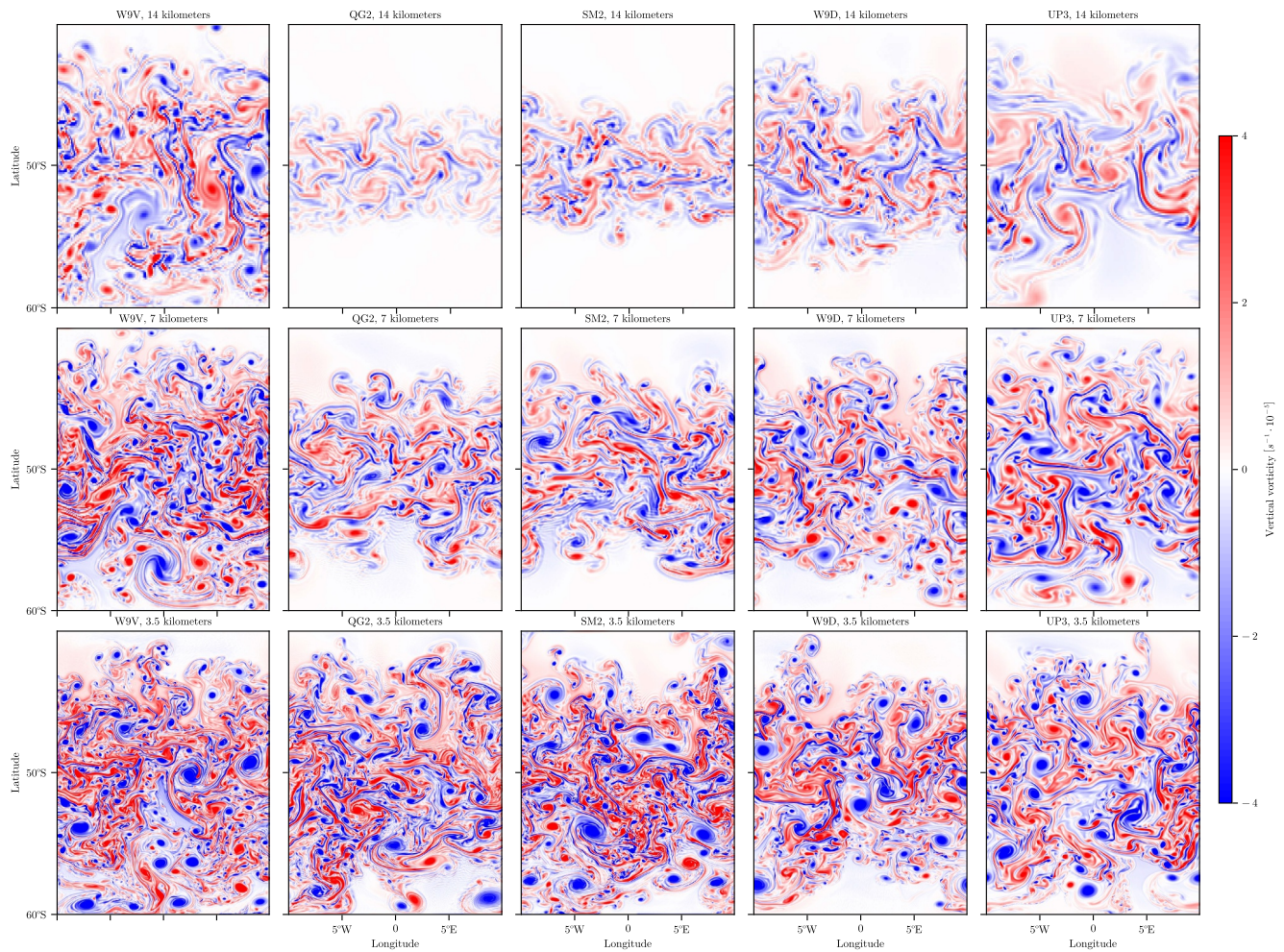
Figure 7. Near-surface vorticity at 14 (top panels), 7 (center panels), and 3.5-km (bottom panels) resolution during the initial instability phase (day 230). The leftmost panel shows W9V while the remaining panels (from left to right) are ordered by increasing kinetic energy.
