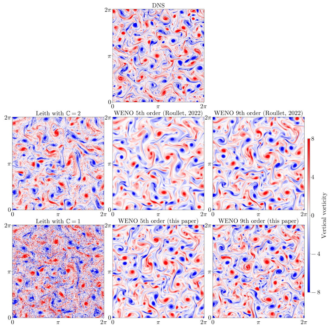
Figure 3. Vorticity at t = 3.6 after initialization. Comparison between Direct Numerical Simulation (top panel), explicit Large Eddy Simulation (LES) with a Leith viscosity (left panels), and implicit LES with a rotational weighted essentially non-oscillatory (WENO) discretization and N = 256^2 . Of the WENO schemes, the top panels show the results obtained with a standard WENO reconstruction of vorticity \{\zeta; \zeta\} (W5D and W9D in Table 1) while the bottom panels show a reconstruction using the velocity field as smoothness measure \{\zeta; \mathbf{u}\} (W5V and W9V in Table 1).
