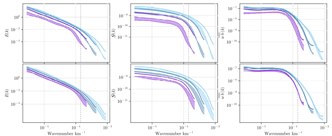
Figure 9. Time-averaged zonal energy spectra (left), enstrophy spectra (center), and w'b' cospectra (right) averaged over the top 200 m. The solid lines are W9V at 14 km (blue), 7 km (steel blue), and 3.5 km resolution (light blue). The banded lines of the same colors show the maximum and minimum trajectory for the dispersive cases (top: SM2, QG2) and diffusive schemes (bottom: UP3, W9D). The vertical dashed line shows the deformation radius.
