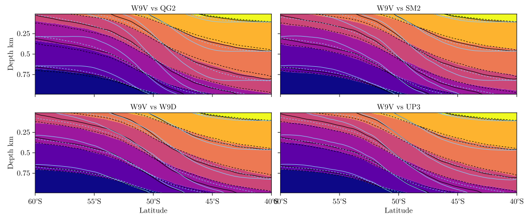
Figure 10. Left: Time and zonally averaged buoyancy for the different cases when compared to W9V. The filled contour shows the results of the comparative case (not W9V) at 3.5-km resolution, acting as a reference, while the dashed and solid contours show solutions at 7 and 14-km resolution, respectively. Black contours are the W9V case, while the light blue show the other case mentioned in the title of each frame (top left: QG2, top right: SM2, bottom left: W9D, bottom right: UP3).
