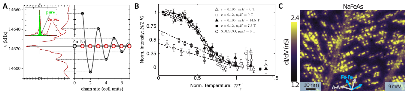
Figure 3. A Zn impurity on 1D inorganic chain YBa 2 NiO 5 [96]. NMR satellite lines (left) indicate different Ni nuclei at different distances from the Zn. Polarization (right) on each site oscillates in sign with distance [88]; B Elastic neutron scattering data on underdoped LSCO showing the intensity at the incommensurate Bragg peaks near (\pi, \pi) vs. temperature T [97]. While a magnetic field induces SDW order, significant incommensurate magnetism is present already in zero field. This effect is enhanced with Zn substitution [98]; C Highly anisotropic electronic states induced by strain near a NaFeAs grain boundary, interpreted as magnetic stripes along the Fe-Fe directions (blue arrows) [99]. (A) Reprinted figure with permission from [88], Copyright 2009 by the American Physical Society. (B) Reprinted figure with permission from [97], Copyright 2008 by the American Physical Society. (C) Reprinted from [99].
