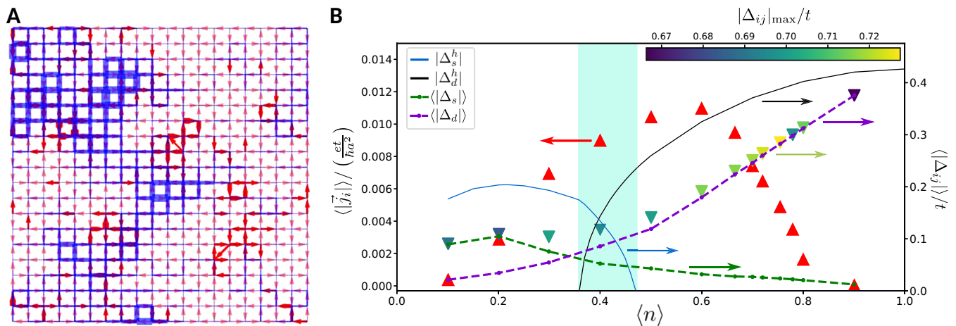
Figure 7. A Spontaneous current pattern in a d -wave superconductor with large disorder [55]. B Zero temperature phase diagram indicating average current (red triangles, left scale) vs. doping. Also indicated are s - and d -wave order parameter amplitudes, respectively (solid lines). The shaded region marks the range of doping where a mixed state s + id is stable in the homogeneous case. Dashed lines show the average d -wave (purple) and s -wave (green) order parameter components (see main text) with random distributions of impurities [56]. (A) Reproduced from [55]. CC BY 4.0. (B) Reprinted figure with permission from [56], Copyright 2007 by the American Physical Society.
