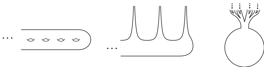
Fig. 1 The Loch Ness monster surface, the flute surface, and the Cantor tree surface
