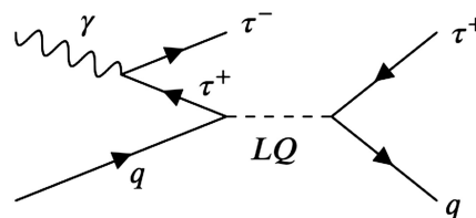
FIG. 1. Feynman diagram of the lepton-induced LQ production.
