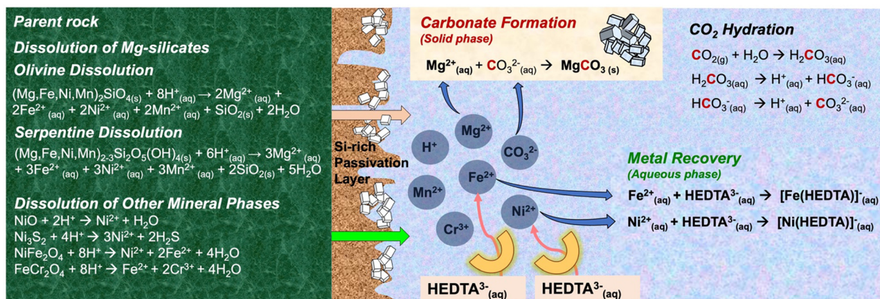
Fig. 1 Schematic representation of the reaction pathways for direct carbon mineralization with concurrent metal recovery.
