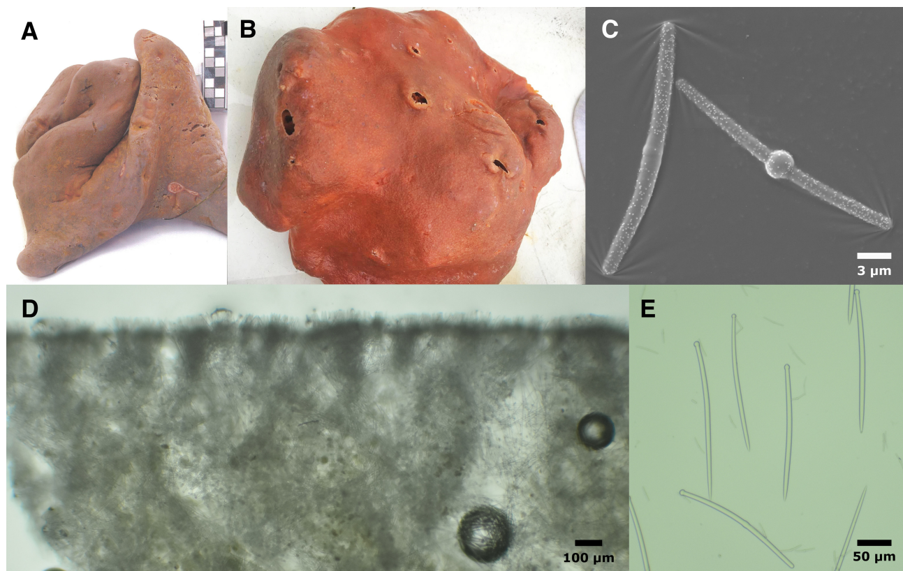
FIGURE 5. Suberites kumeyaay . A–B: Field photos of San Diego Bay sponges before preservation. C: centrotylote microstrongyles. D: Cross-section showing ectosomal brushes and confused interior. E: example tylostyles, including one with slightly off-center head (left), slightly non-terminal head (center) and rare centrotylote strongyle modification (bottom). C–E from holotype.
