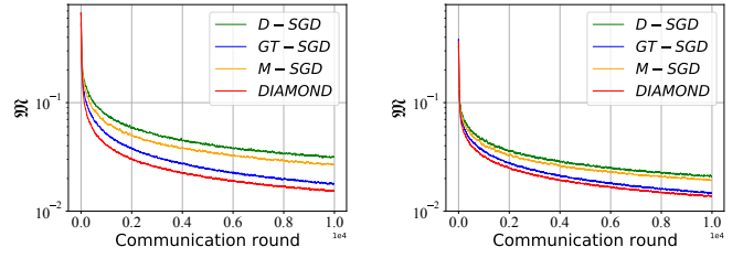
(a) MNIST dataset.
