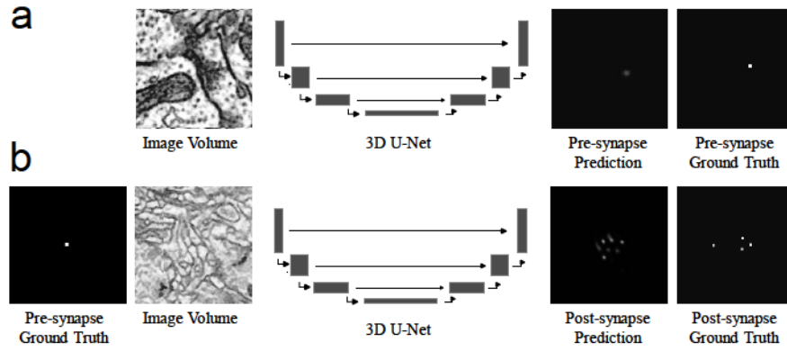
Fig. 4. Baseline method using 3D U-Net. (a) Training of T-bar detection network. The input image patches, subvolumes of ground truth image volumes, are randomly sampled so that some image patches might not contain any T-bar. (b) Training of post-synapse detection network. The T-bar is in the center of each input image patch and a fixed patch will while both the image patches and network are 3D and of isotrop
