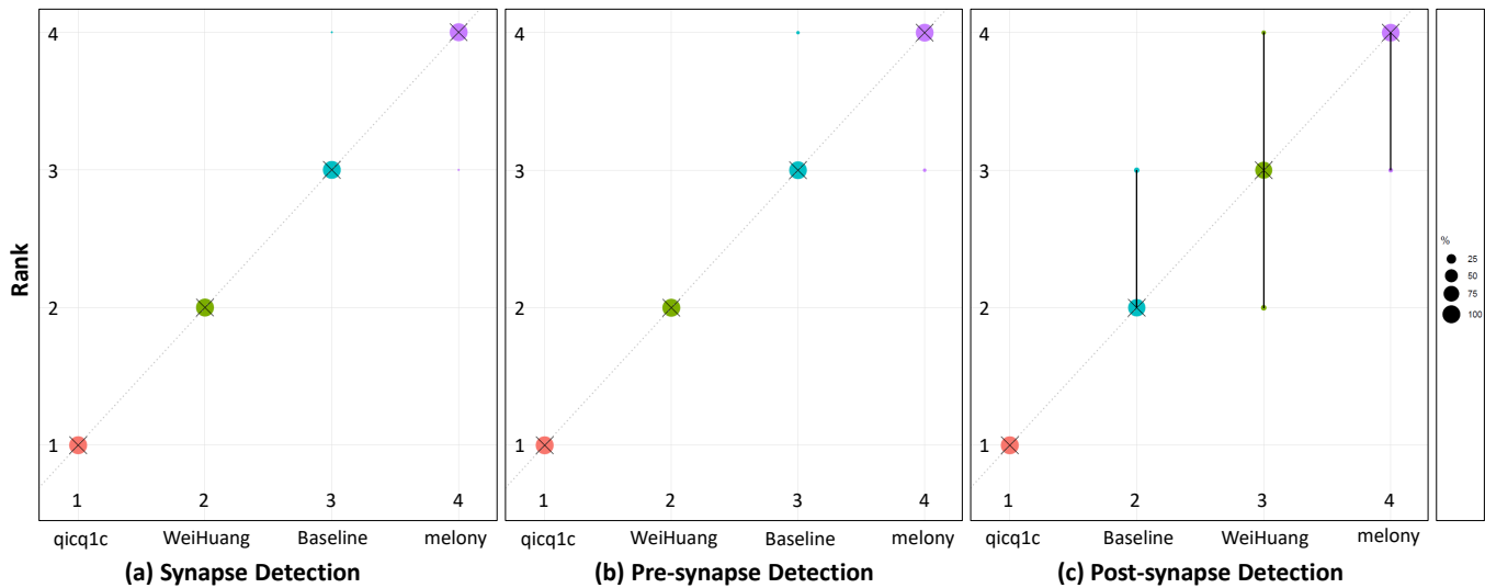
Fig. 9. Ranking uncertainty analysis. Methods are color-coded, and the area of each blob at position (method i , rank j ) is proportional to the relative frequency method i achieved rank j across b = 1000 bootstrap samples. Black cross: the median rank for each method. Black lines: 95% bootstrap intervals across bootstrap samples.
