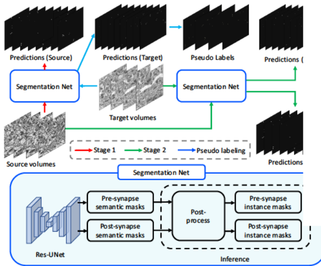
Fig. 5. The framework proposed by Team qicq1c [59]. In the first stage, the team trained an initial segmentation network using the source domain volumes with ground truth labels. In the second stage, they used the pre-trained network to generate pseudo labels for the target domain volumes. Then, the segmentation network is fine-tuned by incorporating both source labels and target pseudo labels as supervision.
