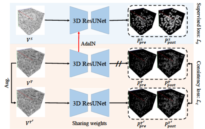
Fig. 6. The framework proposed by Team WeiHuang, consists of Adaptive Instance Normalization (AdaIN) and Consistency Learning (CL). V^S/V^T/V^{T'} : the volume from the source/target/augmented target domain. p_{pre}^S/p_{pre}^T/p_{pre}^{T'} and p_{post}^S/p_{post}^T/p_{post}^{T'} : pre- and post-synapse predictions from the source/target/augmented target volume. Note that the prediction branch of V^T is stop-gradient, i.e., without back-propagation.
