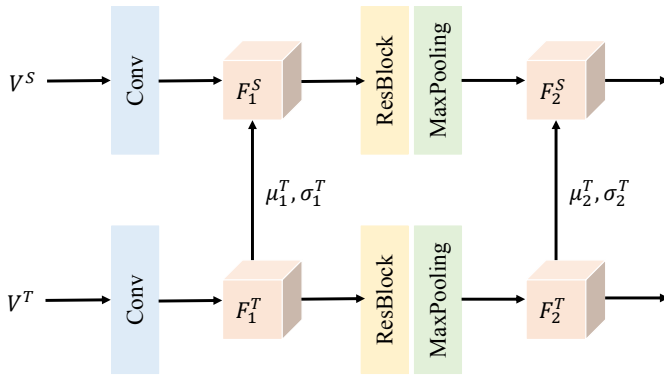
Fig. 7. The structure of AdaIN in the proposed framework by Team WeiHuang. F_i^S/F_i^T : the i -th layer feature in the source/target domain. \mu_i^T and \sigma_i^T : the channel-wise mean and standard deviation of F_i^T .
