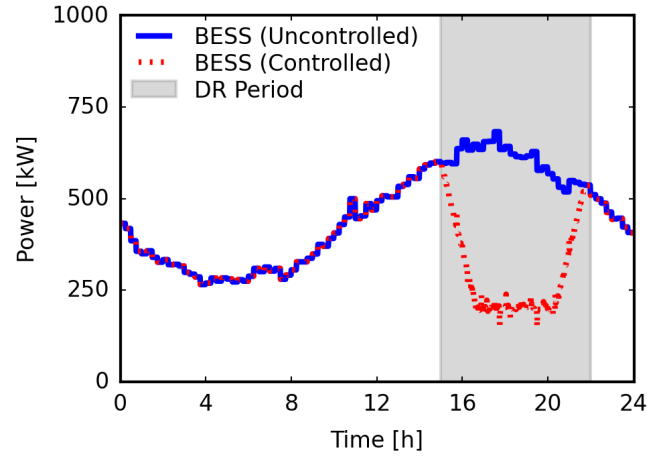
Fig. 4. Discharge of residential battery for DR event from hours 15-22, with gradual increase/decrease at the beginning/end of DR window to decrease ramping. The percentage power reduction for the DR event shown is 22.9%.
