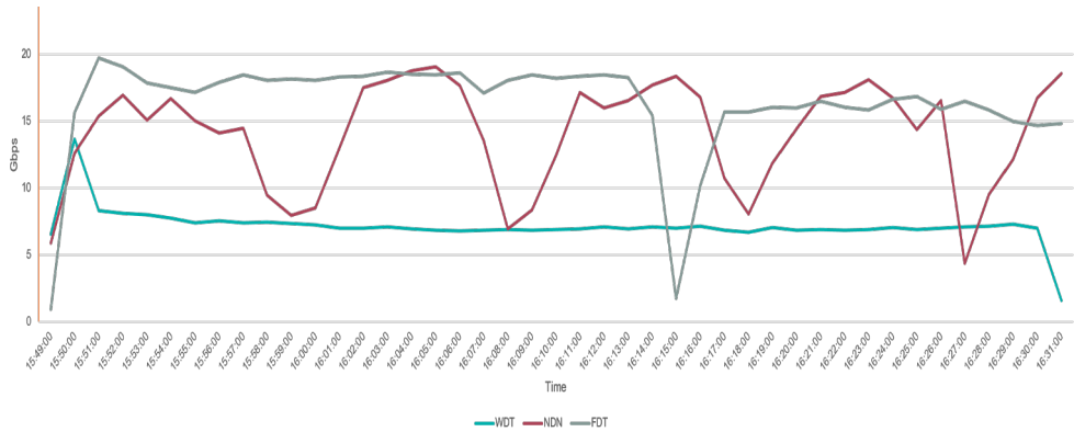
Figure 4: Multi thread WAN transfer (75ms latency, single thread data transfer)
