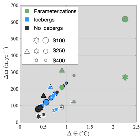
Figure 6. The range of \Theta_z , \Theta_A , and \Theta_{gl} for each simulation ( \Delta\Theta ), plotted with the resulting range of parameterized submarine melt rates ( \Delta\dot{m} ), as defined by Eq. (2). A \Delta\Theta of 0 indicates perfect agreement between \Theta_z , \Theta_A , and \Theta_{gl} for a single run, while a large \Delta\Theta indicates these thermal forcing metrics vary substantially. Iceberg runs are light blue, and non-iceberg runs are gray. White-edged markers depict runs with line plumes, stars represent winter ( Q_{sg} = 10 \text{ m}^3 \text{ s}^{-1} ) simulations, and triangles indicate low-resolution ( Q_{sg} = 1000 \text{ m}^3 \text{ s}^{-1} ) runs. Marker size varies by the sill depth. Green markers depict the range of all seven thermal forcing parameterizations for each sill depth and subglacial discharge group, again plotted against the resultant range of parameterized submarine melt rates. For green markers, a \Delta\Theta of 0 indicates perfect agreement between all seven thermal forcing parameterizations, while a large \Delta\Theta indicates substantial variation between parameterizations.
