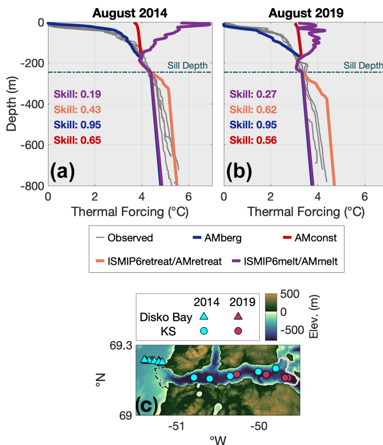
Figure 5. Thermal forcing profiles (gray) observed within Kangeri Sullua (KS) via XCTD casts in (a) August 2014 and (b) August 2019, plotted with the profiles used to calculate ISMIP6retreat (orange) and AMberg (dark blue). The ISMIP6retreat profile is equivalent to external forcing conditions in Disko Bay. Skill score for each parameterization profile is also provided. Horizontal dashed line signifies the maximum depth (245 m) of the Kangeri Sullua entrance sill. (c) Bathymetric map rendering the locations of XCTD casts within Kangeri Sullua (circles) used in (a) and (b), as well as XCTD and CTD casts in Disko Bay (triangles) used to provide external forcing conditions. Solid rose line depicts the Sermeq Kujalleq terminus position in July 2014 (Goliber et al., 2022), and the dashed black line outlines the location of the entrance sill.
