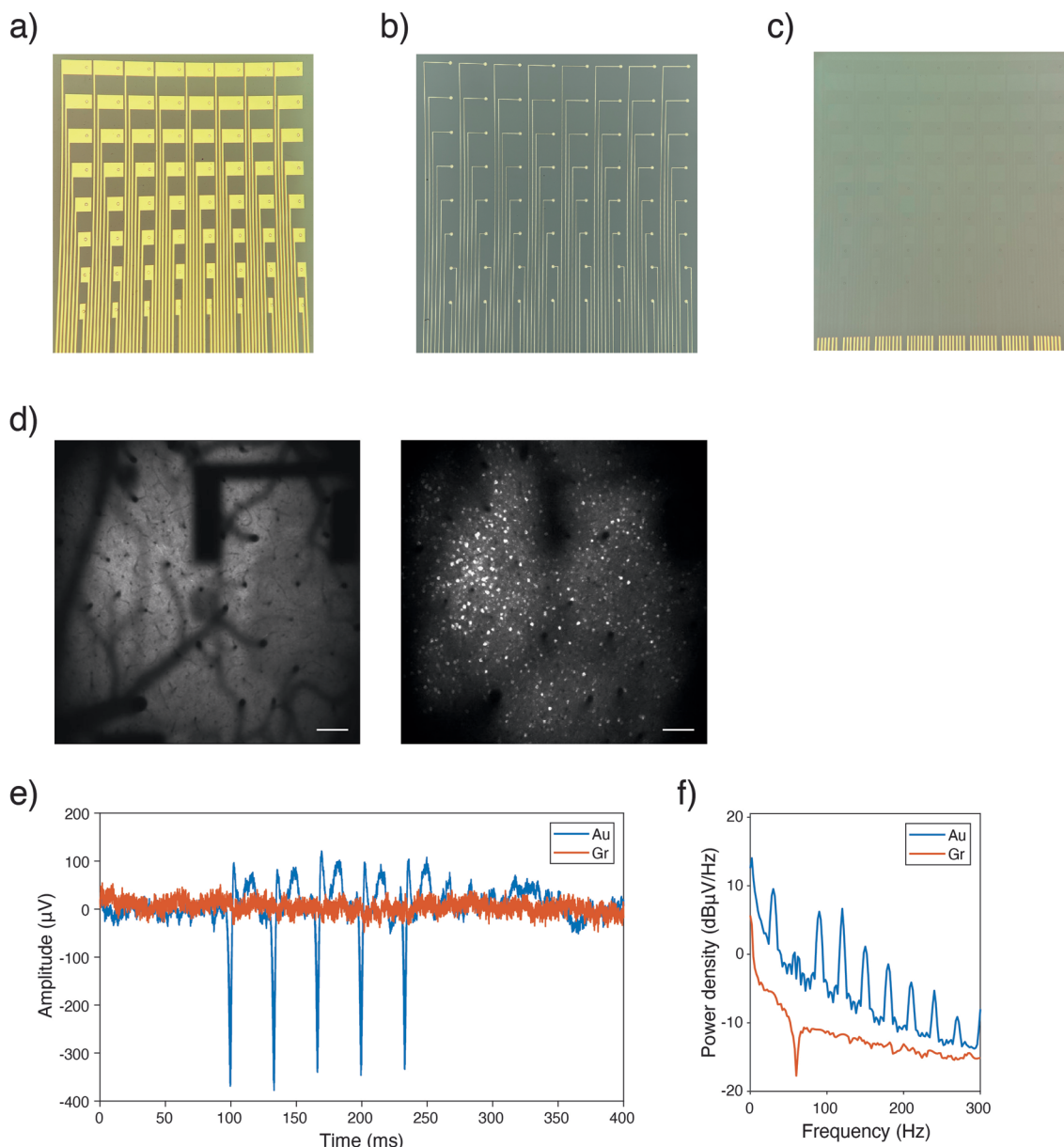
Extended Data Fig. 2 | Comparison of conventional gold electrodes with transparent graphene arrays. (a) Conventional 64-channels gold array with 20 μm and (b) 6 μm wire widths and smaller gold pads. (c) Fully transparent 64-channels graphene array without surrounding gold wires. (d) Shadows created by opaque gold wires in the field of view during two-photon imaging at 50 μm (left) and 250 μm (right) depth under the electrodes. The scale bars are
