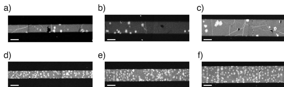
Extended Data Fig. 3 | Characterization of defects in SLG and DLG wires. (a) SLG and DLG wire pinhole images using two-photon microscopy. SLG wire with different width 20 \mu\text{m} , (b) 30 \mu\text{m} , and (c) 40 \mu\text{m} . DLG wire with different width (d) 20 \mu\text{m} , (e) 30 \mu\text{m} , and (f) 40 \mu\text{m} . Scale bars are 20 \mu\text{m} .
