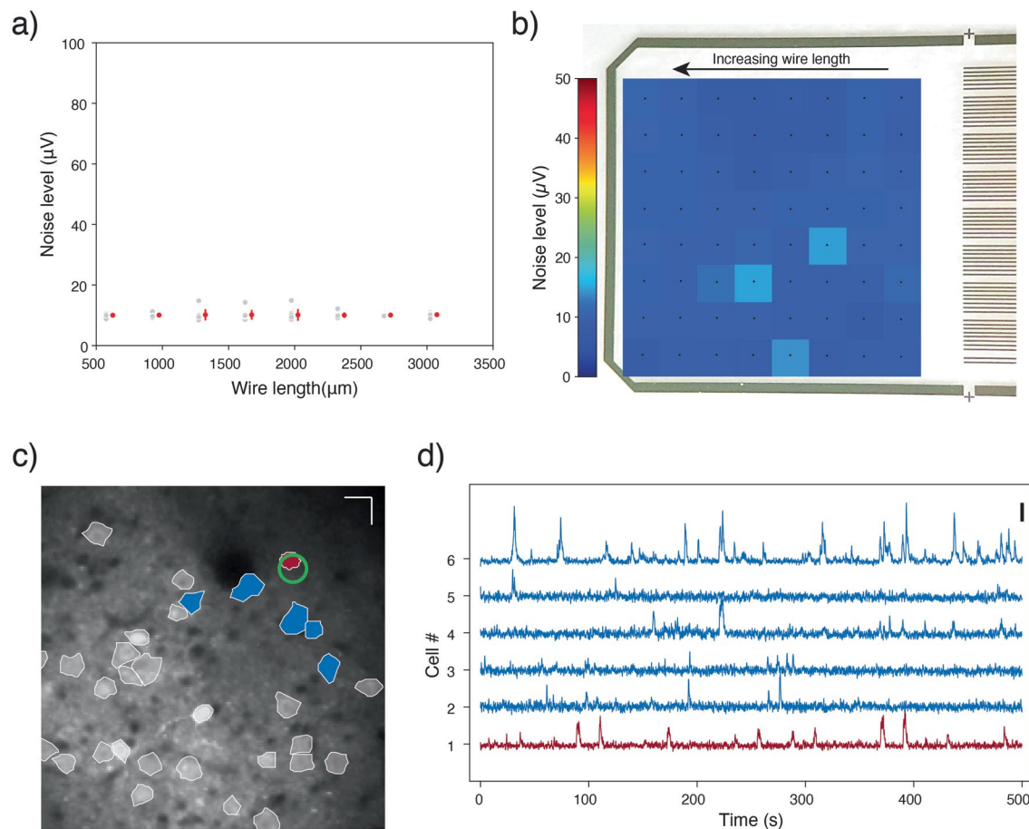
Extended Data Fig. 5 | Transparent graphene arrays do not affect the signal quality. (a) The noise level of all channels with different graphene wire lengths. The gray dots in the graph represent the noise level for individual channels, while the red dots and lines represent the mean and standard deviation of each group of eight channels with same graphene wire length. (b) The heatmap of noise
