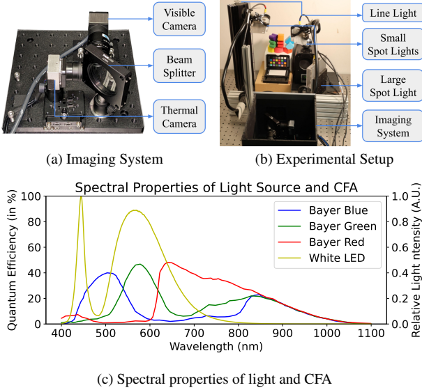
Figure 2. Our imaging system consists of a visible camera and a thermal camera collocated using a gold dichroic beamsplitter. The light sources are placed close to the target scene so that the rise in temperature due to light absorption is detectable in the thermal camera. All the light sources have the same emission spectrum. The relative emission spectrum of the white LED and the quantum efficiency curves of the Color Filter Array are obtained from the corresponding datasheets.
