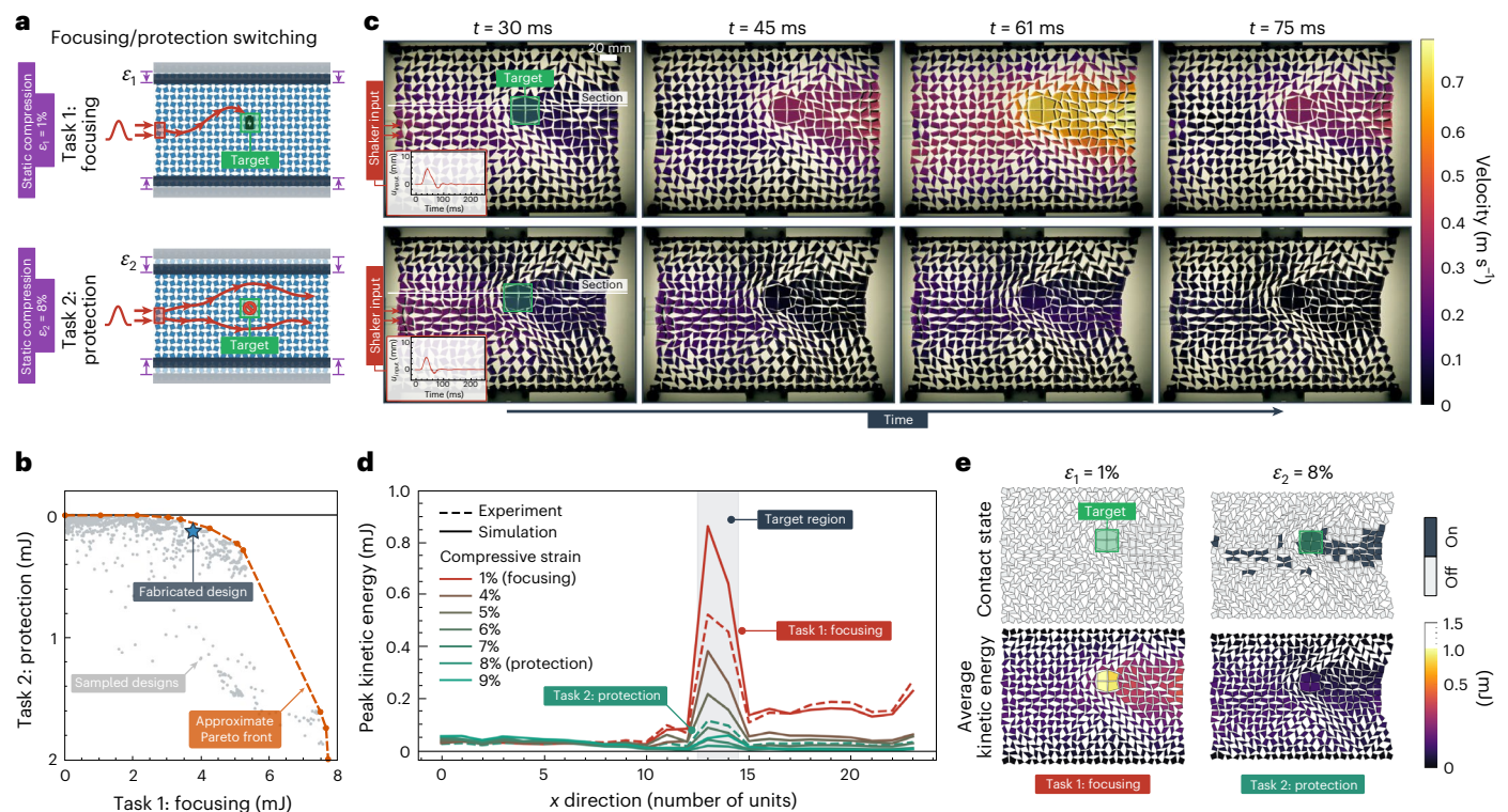
Fig. 4 | Reprogramming functionality. a , We search for a metamaterial architecture with the ability to maximize kinetic energy at a target location for an applied precompression of \varepsilon_1 = 1\% (top) and minimize it for \varepsilon_2 = 8\% (bottom). b , All designs visited during optimization (grey points) plotted in the objective space J_{\Omega_1}^{(\varepsilon_1)}/t_f - J_{\Omega_2}^{(\varepsilon_2)}/t_f . The resulting Pareto front is highlighted by the orange dashed line. c , Experimental snapshots of the fabricated design (marked by a blue star in b )
