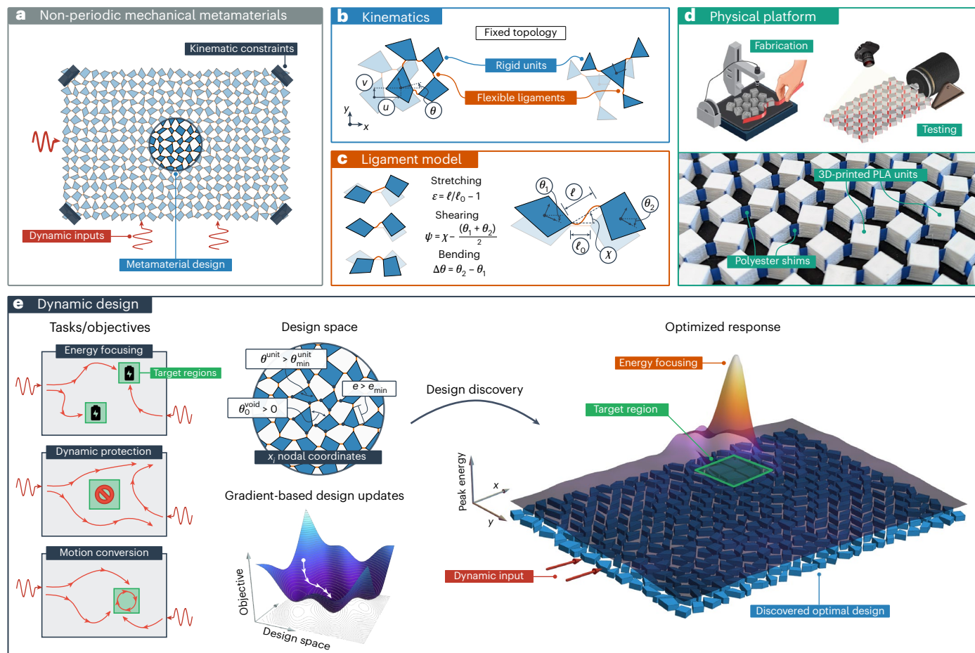
Fig. 1 | Automated design of reprogrammable nonlinear dynamic
